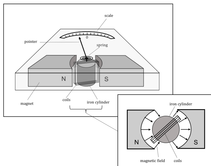
Figure 427: Illustration of a galvanometer. Current passes through the coil, and the coil rotates due to the torque from a magnetic field created by a permanent magnet. The torque from the magnetic force is balanced by a torsional spring.
