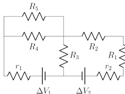
Figure 391: A circuit that can be simplified and then solved with Kirchhoff's rules.
