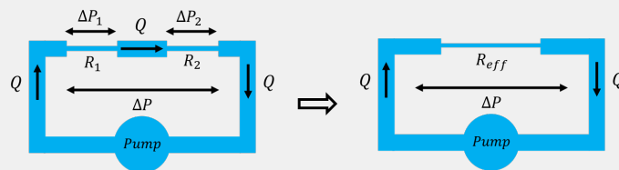
Figure 371: Left panel: What a series circuit would look like in the context of fluid mechanics. Right panel: The two resistors can be thought of as a single resistor with effective resistance R_{eff} = R_1 + R_2 .
