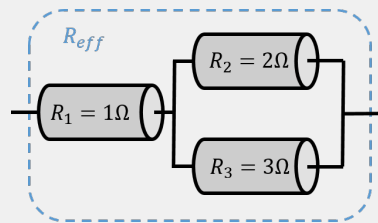
Figure 374: A combination of three resistors.
