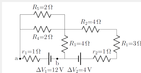
Figure 396: The same circuit as in Figure 16 , with values filled in.
