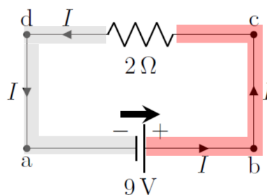
Figure 380: The same circuit as in Figure 4 showing the two regions over which the electric potential is constant.
