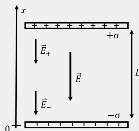
Figure 353: Two parallel plates with equal and opposite surface charge densities. In the region between the plates, the electric field is uniform.
