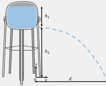
Figure 289: Water leaking out of a horizontal hole in a water tank.
