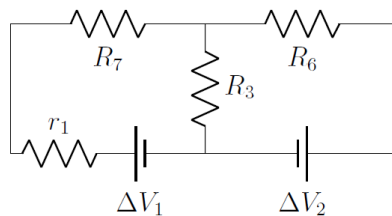
Figure 393: The resistors R_4 and R_5 in parallel from the circuit in Figure 17 have been combined into the effective resistor, R_7 , to simplify the circuit.
