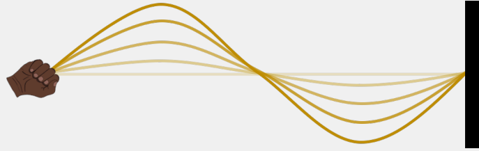
Figure 264: A standing wave as a stationary wave whose amplitude changes over time
