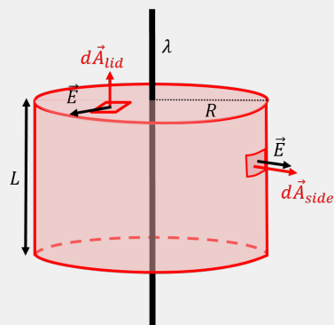
Figure 338: A cylindrical Gaussian surface is used to calculate the flux from an infinite line of charge.
