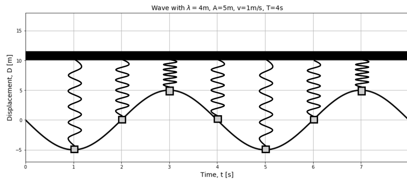
Figure 257: The displacement as a function of time for one particle in the medium (at x = 0 ) is identical to the motion of a simple harmonic oscillator.
