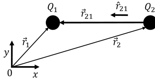
Figure 301: Vectors involved in applying Coulomb's Law.
