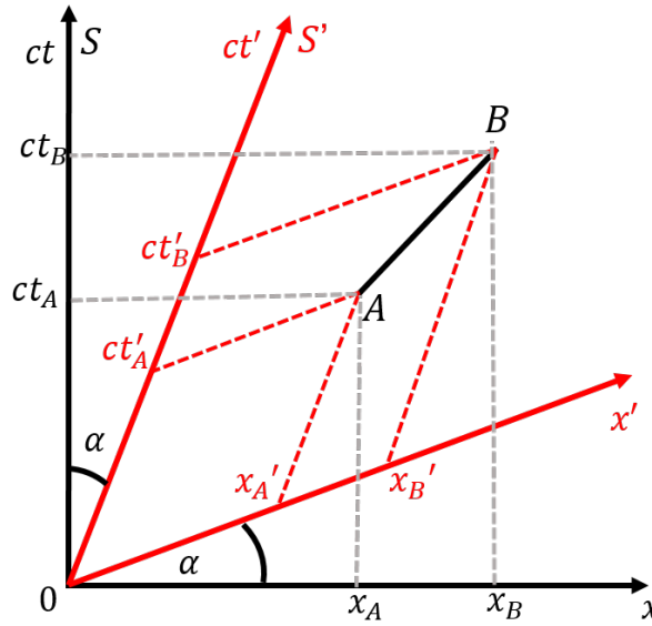
Figure 485: The reference frame S' is moving relative to reference frame, S , with speed v in the x direction. We can illustrate this on a space-time diagram by tilting the axes of the S' coordinate system by an angle \tan \alpha = v/c , as shown.
