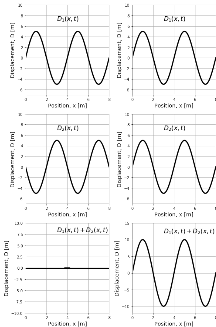
Figure 262: Destructive (left) and constructive (right) interference of waves.
