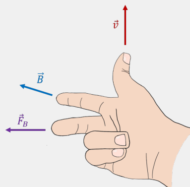
Figure 413: The way that Josh remembers the right hand rule for magnetism.
