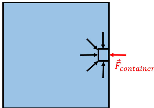
Figure 271: At the edge of a container, a small element of fluid will exert an outwards force on the container, and the container will exert an inwards force on the element of fluid.
