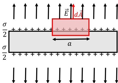
Figure 344: Cross-section of a conducting plane where the charges migrate to the surface. A box-shaped Gaussian surface is also shown as seen from the side (the third dimension of the box is perpendicular to the plane of the page).
