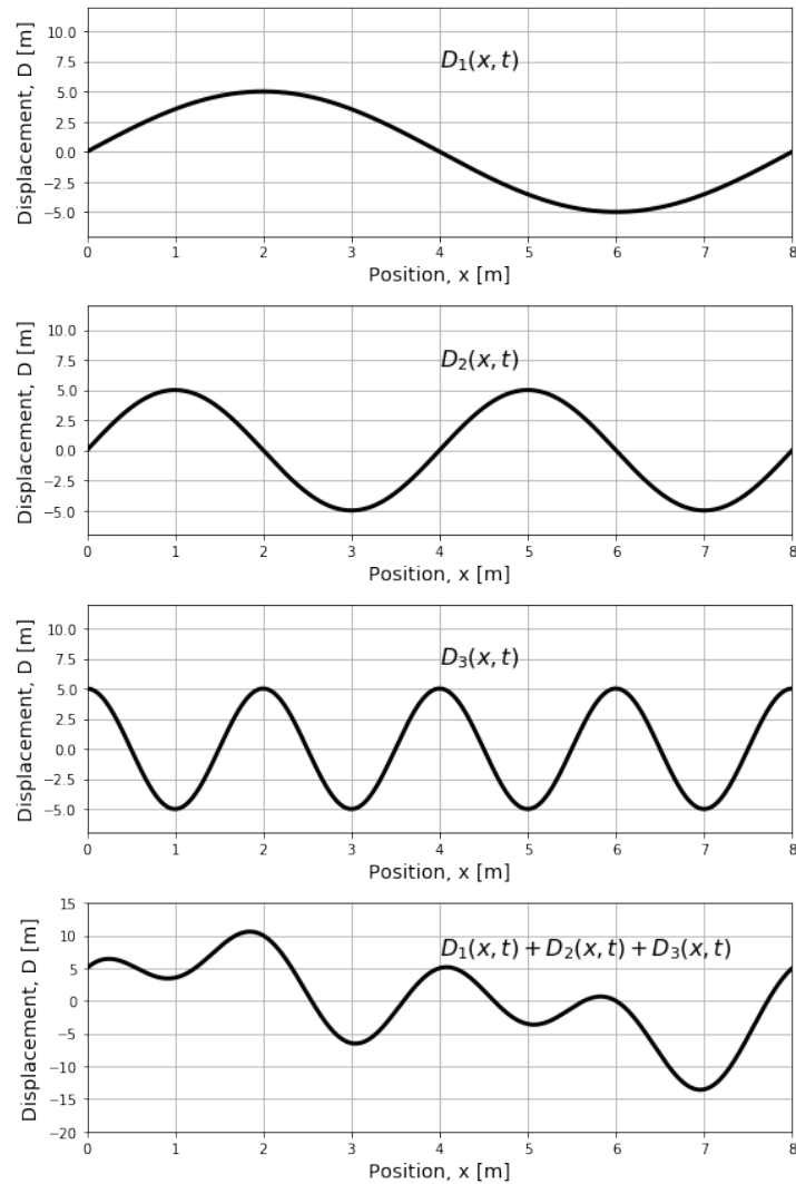
Figure 261: The superposition of three waves to create a resulting wave shown in the bottom panel. The waves are shown as the displacement as a function of position at a fixed instant in time.
