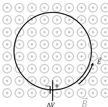
Figure 462: A varying magnetic field will induce a circular electric field.
