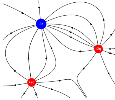
Figure 309: Field lines of two +2q charges and one -3q charge.
