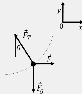
Figure 149: A free-body diagram of the forces exerted on the child.
