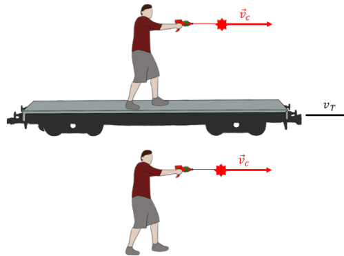
Figure 472: Two people fire a laser pulse. Regardless of whether the pulse of laser light was fired from a moving train or from the ground, it will have a speed of c in all frames of reference.
