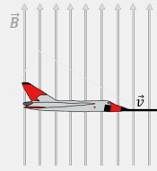
Figure 467: The Avro Arrow moving through a magnetic field.
