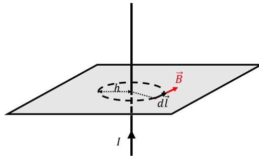
Figure 443: An Amperian loop that is a circle of radius, h , will allow us to determine the magnetic field at a distance, h , from an infinitely-long current-carrying wire.
