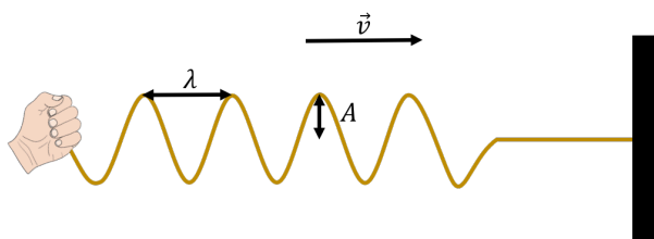
Figure 249: Wavelength, velocity, and amplitude for a transverse wave on a rope.
