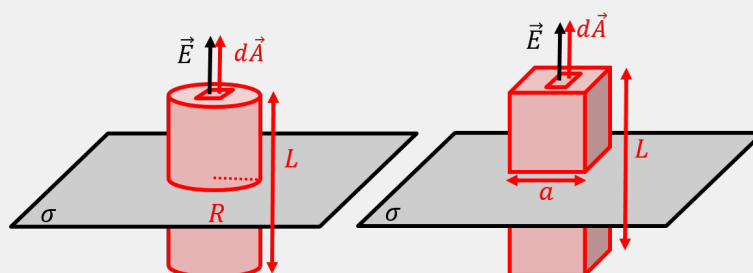
Figure 343: A cylindrical surface or a box are both good choices for a Gaussian surface above a plane, since only the parts of the surface parallel to the plane will have net flux through them.
