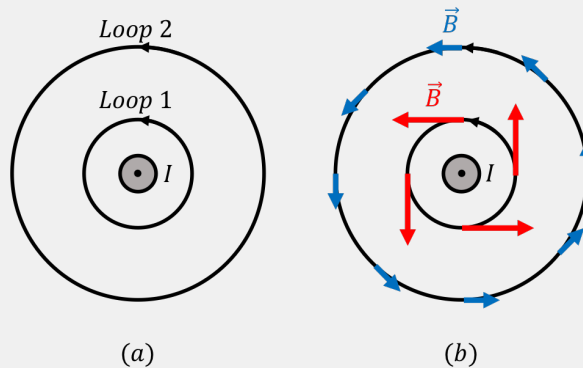
Figure 444: Left: 2 Amperian loops around a current carrying wire. Right: Magnetic field vectors around each loop.
