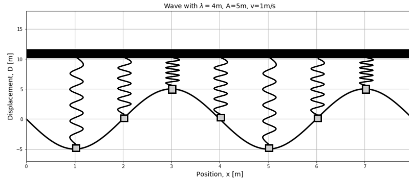
Figure 258: The displacement as a function of position for different points in a medium. Each point in the medium can be modelled as a simple harmonic oscillator.
