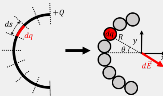
Figure 312: Left: Cutting up a wire with charge Q into pieces with length ds and charge dq . Right: Visualizing the semicircular wire as being made up of point charges.
