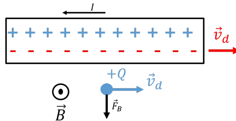
Figure 480: A positive charge, +Q , moving towards the right, near a wire carrying current towards the left, will experience a downwards magnetic force, \vec{F}_B = Q\vec{v}_d \times \vec{B} .
