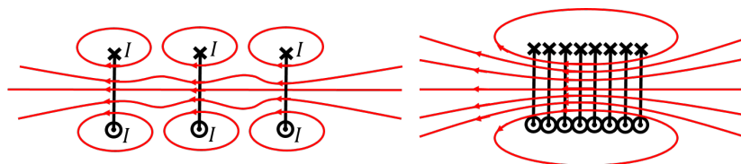
Figure 448: As multiple loops of current are brought together to form a solenoid, the magnetic field inside the solenoid becomes uniform and the field outside the solenoid approaches zero.
