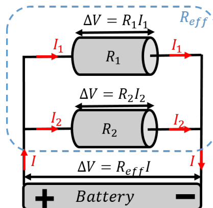
Figure 372: When two resistors are connected in parallel, the same voltage is applied across each resistor.
