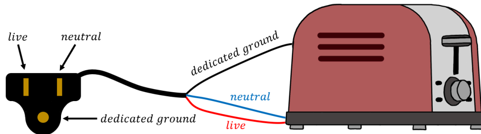
Figure 375: When an appliance has three prongs on its electrical cable, the middle prong grounds the case to the dedicated ground as a safety measure. Note that the live wire is not necessarily the right-hand side socket on an outlet!
