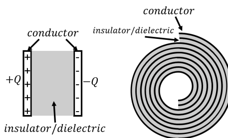
Figure 360: Two examples of capacitors. The left panel shows a “parallel plate” capacitor, and the right panel shows a cylindrically shaped capacitor obtained by “rolling up” a parallel plate capacitor.
