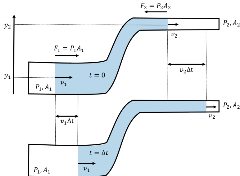
Figure 286: Laminar flow of an incompressible fluid through a pipe that changes cross-sectional area and height in the direction of flow. An element of fluid, in blue, is shown at time t = 0 (top panel), and then, at a later time, t = \Delta t (bottom panel).
