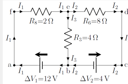
Figure 397: Simplified version of the circuit in Figure 21.
