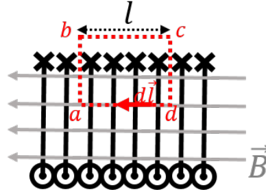
Figure 449: We use Ampère's Law with a rectangular loop to evaluate the strength of the magnetic field inside a solenoid.
