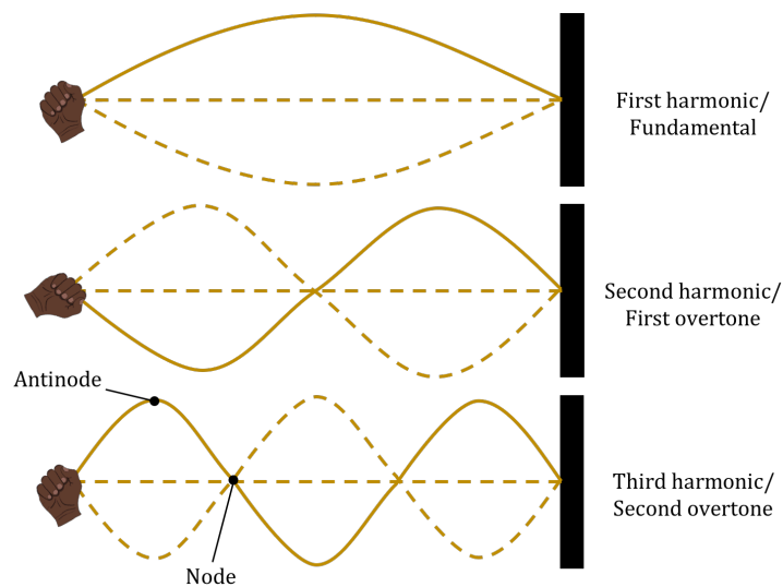
Figure 263: The first three standing waves on a string.
