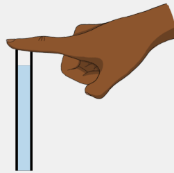
Figure 273: Holding water in a vertical straw.
