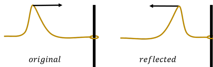
Figure 254: When the end of the rope is free, the reflected pulse will be upright.
