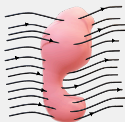
Figure 328: A non-uniform electric field flowing through an irregularly shaped closed surface.
