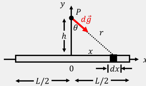
Figure 184: A thin rod of mass M and length L produces a gravitational field at a point P located above the midsection of the rod. Each segment of the rod dx will contribute to the gravitational field.
