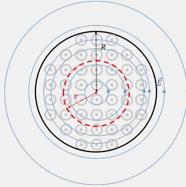
Figure 463: The induced electric field lines form closed circles when the magnetic field changes.
