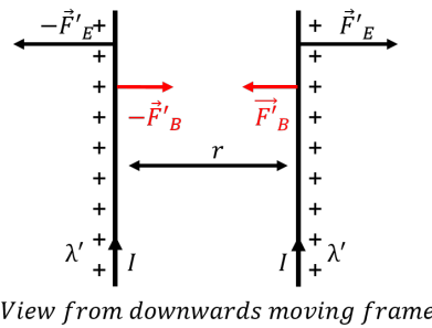
Figure 469: Two infinitely-long charged wires as viewed from a down-going frame of reference will appear to have upwards-going currents that will result in an attractive magnetic force between the wires.
