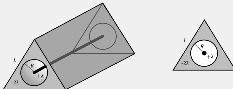
Figure 346: Left: Wire surrounded by a conducting shell with a cylindrical inner surface and triangular outer surface. Right: Cross section of the set-up.
