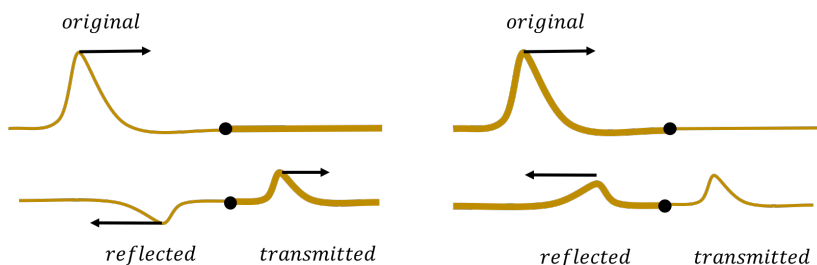
Figure 255: A pulse can be both reflected and transmitted as it changes medium. Left panel: The pulse is transmitted from a lighter rope to a heavier rope. Right panel: The pulse is transmitted from a heavier rope to a lighter rope
