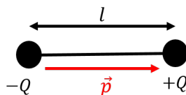
Figure 320: An electric dipole and its corresponding dipole vector, \vec{p} .
