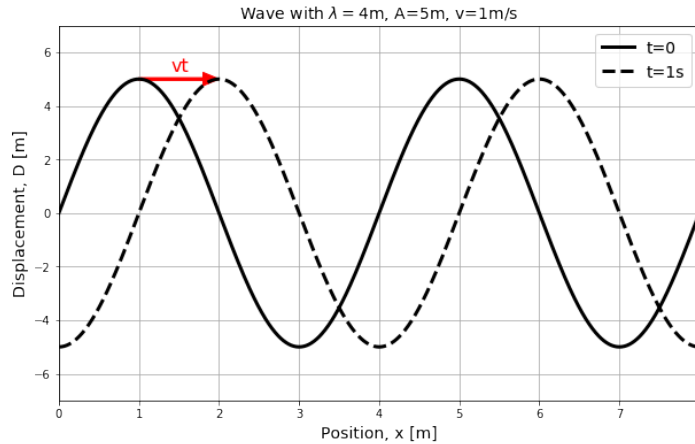
Figure 251: Displacement as a function of position for particles in a medium as a wave passes through. The dotted line shows the displacement as a function of time upright 1/s after the solid line, and corresponds to a wave travelling towards the right.
