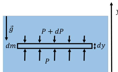
Figure 274: Pressure gradient from gravity on an infinitesimal fluid element.
