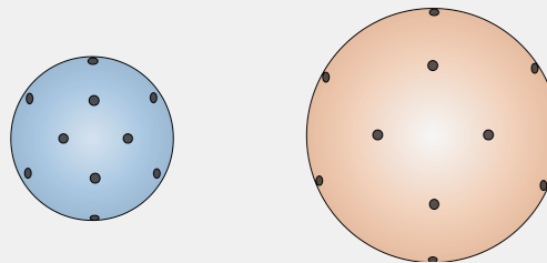
Figure 335: The Gaussian surfaces from Figure 10, where the dots show where the field lines passed through each surface.
