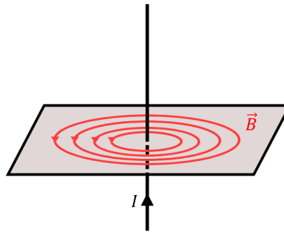
Figure 435: The magnetic field from a current-carrying wire forms concentric circles centred on the wire.
