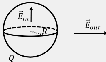
Figure 330: For a spherical charge distribution, the electric field inside and outside must point in the radial direction, by symmetry.
