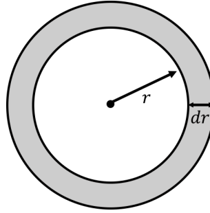
Figure 260: A spherical shell at radial position r with thickness dr
