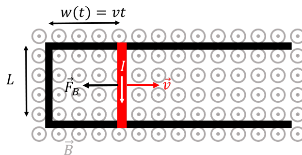
Figure 459: A U-shaped rail on top of which a bar of length, L , can slide. The system is immersed in a magnetic field that points out of the page. The bar moves to the right with a constant speed, v .
