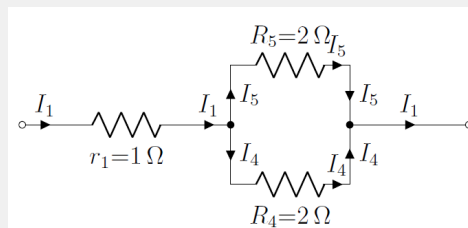
Figure 398: The components of the effective R_8 resistor from Figure 22 . The current, I_1 , coming from the battery goes through r_1 and then splits up.
