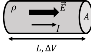
Figure 369: A simple resistor of length, L , cross-sectional area, A , made from a materials with resistivity, \rho . A potential difference, \Delta V , is applied across the resistor, leading to an electric field and current in the resistor.
