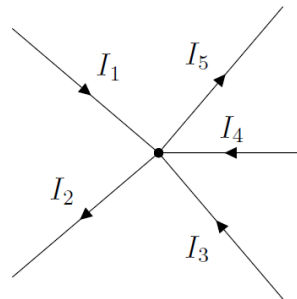
Figure 388: A junction with 5 segments and 5 currents.
