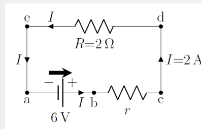
Figure 385: A circuit showing a real battery (with internal resistance r ) in series with a resistor.
