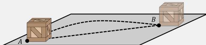
Figure 154: You push a crate from A to B along any path.
