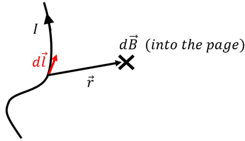
Figure 433: The infinitesimal magnetic field, d\vec{B} , that is created by an infinitesimal section of wire, d\vec{l} , carrying current I . Note that the vector, \vec{r} , goes from d\vec{l} to the point where we wish to calculate the field.
