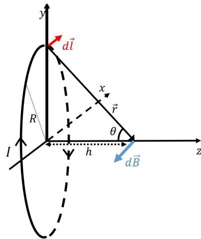
Figure 437: Diagram to apply the Biot-Savart Law in order to determine the magnetic field along the symmetry axis of a ring carrying current, I . The x axis goes into the page.
