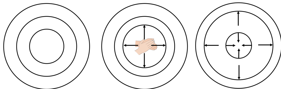
Figure 259: Left: We divide the air into thin spherical shells. Here we represent three shells (the black circles). Center: When you clap, the innermost shell is given energy and expands. Right: Energy is transferred to the next shell, which expands as the first
