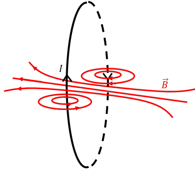
Figure 436: The magnetic field from a current-carrying loop of wire can be thought of as the sum of the fields from small straight sections of wire.
