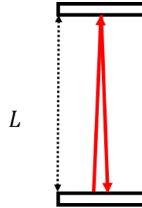
Figure 475: A clock is made by having a pulse of light bounce back and forth between two parallel mirrors separated by a distance, L .
