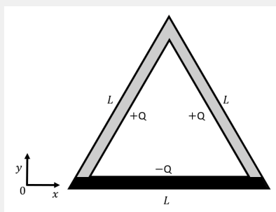
Figure 323: A triangle made up of charged rods
