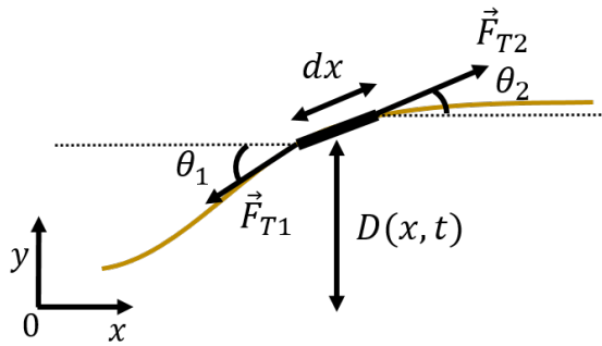
Figure 256: A small section of rope under tension as a wave passes through.
