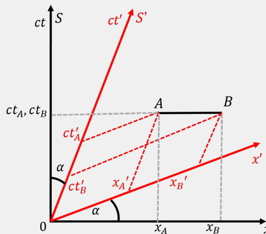
Figure 486: In the frame of reference S , the events A and B occur at the same time. In frame, S' , event B occurs before event A (since t_B < t_A ). The two events are space-like, so observers in different frames of reference cannot agree on which happened first.
