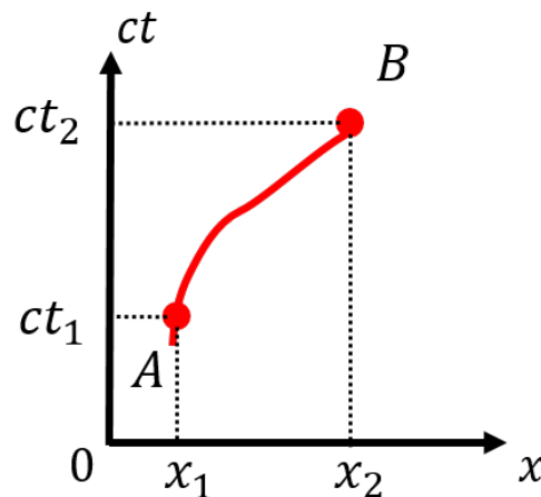
Figure 482: World line of an object that moved from locations A in space-time to location B in space-time.
