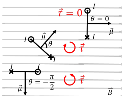
Figure 423: Three loops of current with different orientations relative to a uniform magnetic field. The loops are seen from above, and the current is shown coming in and out of the page on each loop, along with the corresponding magnetic dipole moment vector.
