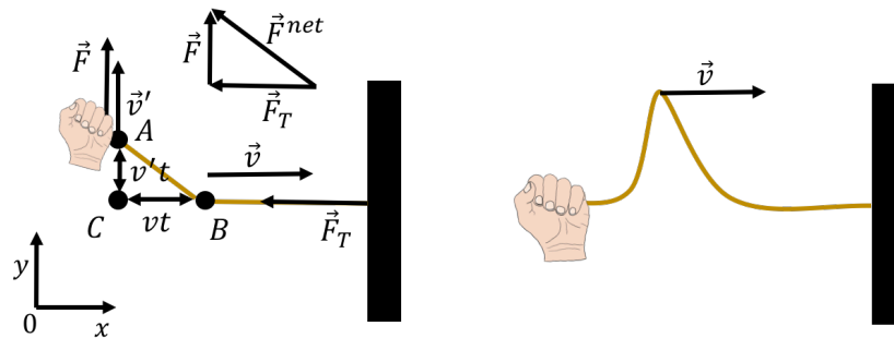
Figure 252: (Left:) Pulling upwards and then downwards on a horizontal rope causes a pulse to form and propagate. After a short period of time, a pulse is seen propagating down the rope (right).
