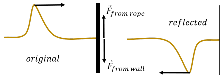
Figure 253: When the end of the rope is held fixed, the reflected pulse will be inverted.
