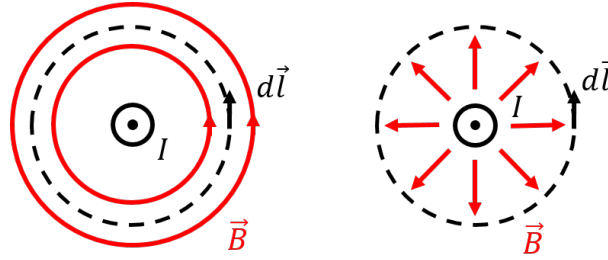
Figure 442: By symmetry, the magnetic field from a current-carrying infinite wire (illustrated with current coming out of the page), must either form concentric circles (left panel), or be in the radial direction (right panel). We know that the former (circles, left panel) is the correct choice. The dotted lines show “Ampèrian loops” that one can use to calculate the integral in Ampère’s Law.
