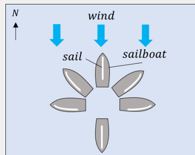
Figure 269: Possible directions you can point your sailboat.
