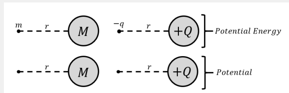
Figure 350: Gravitational potential energy and gravitational potential (left) next to its electrical analogue (right).
