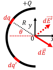
Figure 311: Infinitesimal electric fields from point charges along the bent wire.
