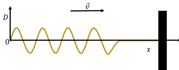
Figure 250: The displacement ( D ) of points at different positions ( x ) on a rope as a sine wave passes through.
