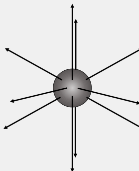
Figure 333: The field lines for a positively charged sphere.
