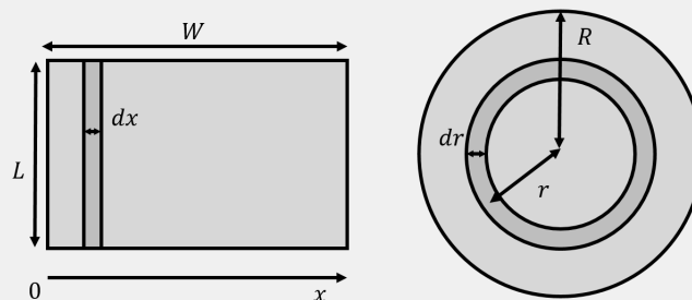
Figure 316: A two-dimensional object such as a plane modelled as a the sum of infinitely thin lines (left panel) or as the sum of infinitely thin rings (right panel).
