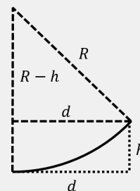
Figure 431: Deflection of an electron moving in a uniform magnetic field.
