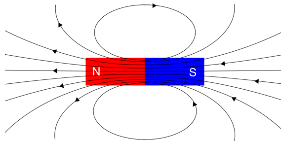
Figure 411: The magnetic field lines for a bar magnet always form closed loops as they do not end at the North or South pole of the magnet.
