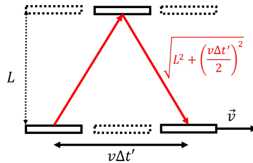
Figure 476: A clock is made by having a pulse of light bounce back and forth between two parallel mirrors separated by a distance, L . When the clock is placed on a spaceship moving with speed, v , the light travels a longer distance before completing a full cycle, as observed by someone not travelling with the clock.
