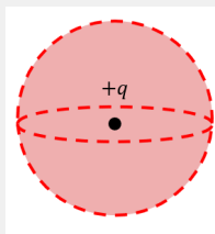
Figure 340: . A spherical Gaussian surface to enclose a point charge.
