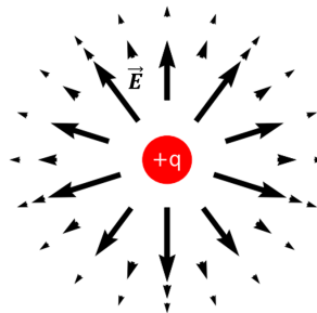
Figure 307: Electric field vectors near a point charge.
