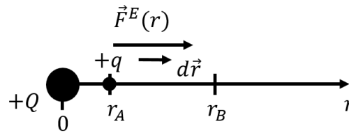
Figure 348: Calculating the work done on a charge +q by the electric force exerted by charge +Q when charge +q moves from a distance r_A to a distance r_B from the centre of charge +Q .
