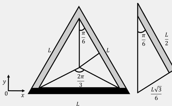
Figure 324: Solving for \theta_0 and R
