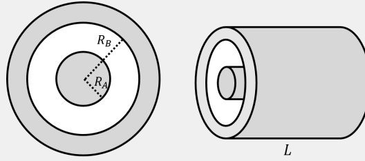
Figure 362: A capacitor constructed from concentric cylinders.
