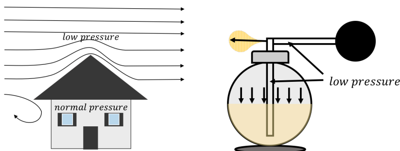
Figure 288: (Left:) the wind flowing above a roof creates a low pressure zone above the roof. (Right:) air flowing above a vertical spout in the atomizer creates a low pressure zone; the air pressure in the bottle forces the liquid up the spout.
