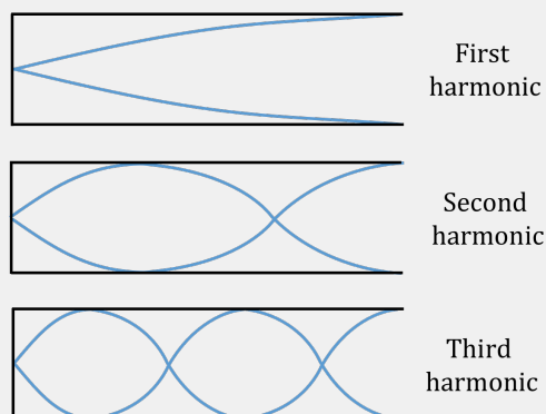
Figure 267: The first three harmonics for a clarinet. There is a node at the fixed end and an anti-node at the free end.
