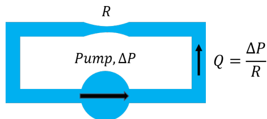
Figure 381: A fluid dynamics analogue of the circuit in Figure 4 , where a pump plays the role of the battery, and a narrow pipe that of a resistor.
