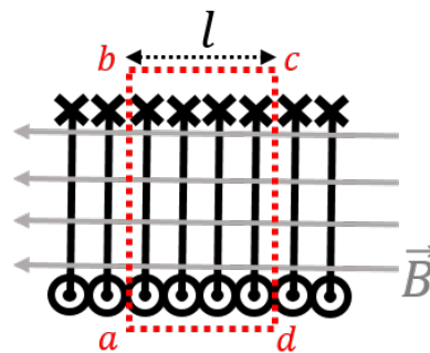
Figure 450: By extending the Amperian loop to both sides of the solenoid, we conclude that the magnetic field just outside the solenoid must be zero, because the net current enclosed is zero.
