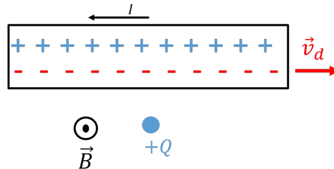
Figure 479: A stationary positive charge, +Q , near a wire carrying current towards the left. This leads to a magnetic field out of the page at the location of Q .
