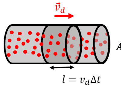
Figure 367: A section of electrons of length l drifting through a conductor of cross-sectional area, A .
