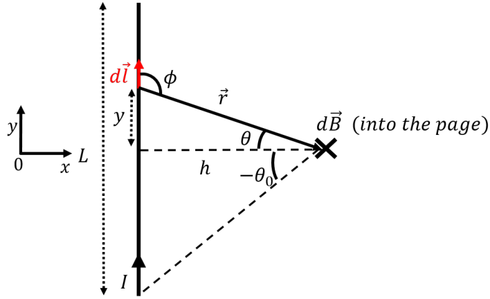
Figure 434: Setting up the model to use the Biot-Savart Law to calculate the magnetic field a distance h from the centre of a current-carrying wire of length L .
