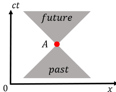
Figure 483: The past and future light cones associated with the space-time event, A .
