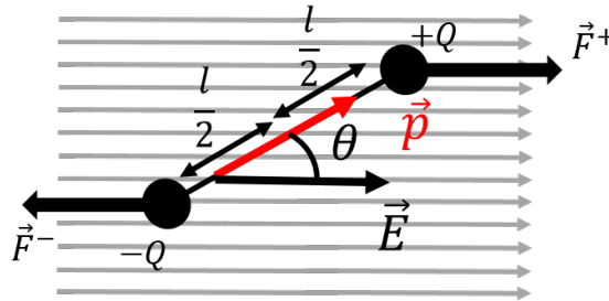
Figure 322: An electric dipole in a uniform electric field.
