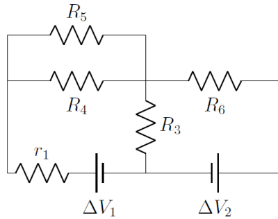
Figure 392: The resistors r_2 , R_1 and R_2 in series from the circuit in Figure 16 have been combined into the effective resistor, R_6 , to simplify the circuit.
