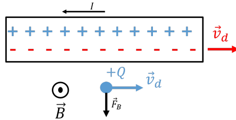
Figure 478: A positive charge, +Q , moving towards the right, near a wire carrying current towards the left, will experience a downwards magnetic force, \vec{F}_B = Q\vec{v}_d \times \vec{B} .
