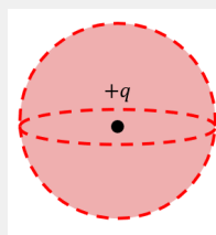
Figure 338: . A spherical Gaussian surface to enclose a point charge.
