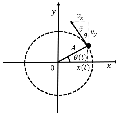
Figure 229: Uniform circular motion of a particle along a circle of radius A with constant angular speed \omega .
