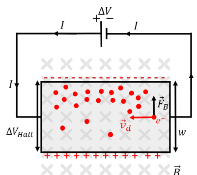
Figure 422: Illustration of the Hall effect, as electrons flow through a slab that is immersed in a magnetic field, the magnetic force pushes them to one side, creating an
