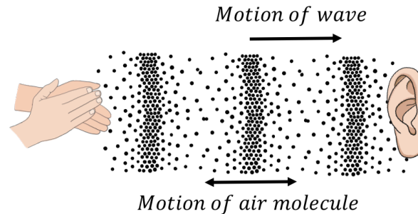
Figure 244: A longitudinal sound wave travelling through the air. The air molecules move back and forth in the same direction as the wave, but they oscillate about an equilibrium position instead of moving with the wave.
