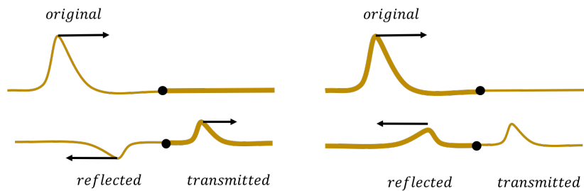
Figure 253: A pulse can be both reflected and transmitted as it changes medium. Left panel: The pulse is transmitted from a lighter rope to a heavier rope. Right panel: The pulse is transmitted from a heavier rope to a lighter rope
