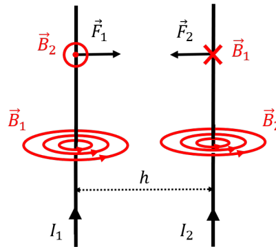
Figure 437: Two parallel current-carrying wires will exert an attractive force on each other, if their currents are in the same direction.
