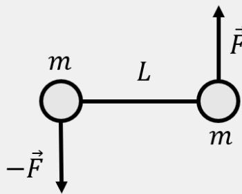
Figure 198: A dumbbell made of two small identical masses separated by a distance L .
