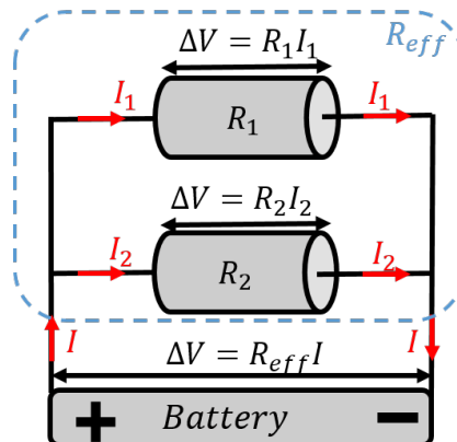
Figure 370: When two resistors are connected in parallel, the same voltage is applied across each resistor.
