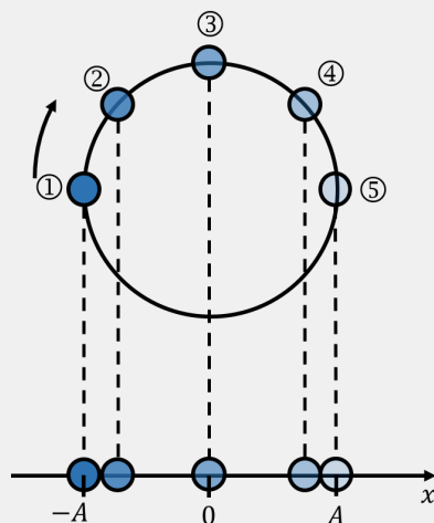
Figure 230: Projecting the motion of a ball around a circle onto the x axis.
