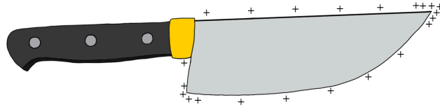
Figure 357: On an uneven conductor, charges will accumulate on the sharper points, where the radius of curvature is the smallest.
