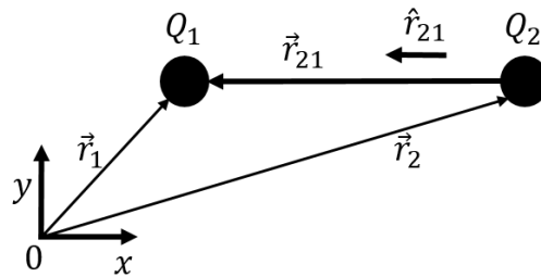
Figure 299: Vectors involved in applying Coulomb's Law.
