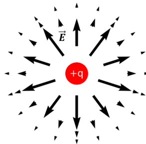
Figure 305: Electric field vectors near a point charge.
