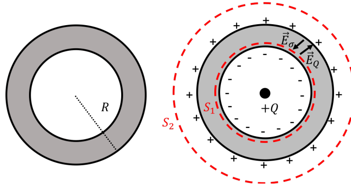
Figure 343: Left: a neutral conducting spherical shell (seen edge on). Right: A positive charge, +Q , placed at the centre of the shell. Charges in the shell will separate in order to keep the electric field inside the conductor zero.
