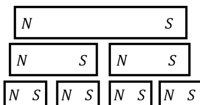
Figure 408: When a bar magnet is cut through the middle, one obtains two magnets, each with a North and South pole, rather than a North and a South magnet.
