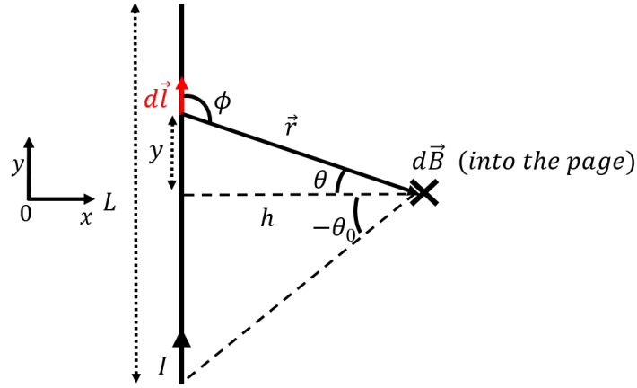
Figure 432: Setting up the model to use the Biot-Savart Law to calculate the magnetic field a distance h from the centre of a current-carrying wire of length L .
