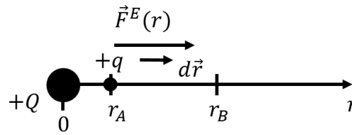
Figure 346: Calculating the work done on a charge +q by the electric force exerted by charge +Q when charge +q moves from a distance r_A to a distance r_B from the centre of charge +Q .
