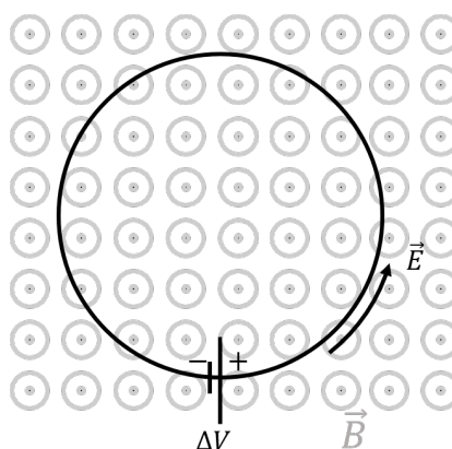
Figure 460: A varying magnetic field will induce a circular electric field.
