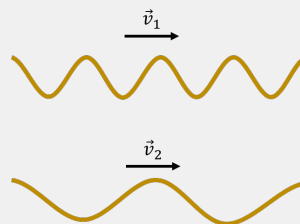
Figure 240: Two waves travelling down two identical strings.
