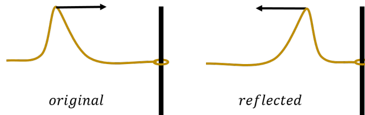
Figure 252: When the end of the rope is free, the reflected pulse will be upright.
