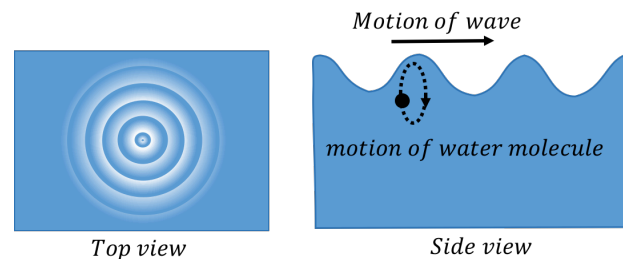
Figure 242: A transverse wave travelling through water. The left panel shows the view from above as ripples move outwards. The right panel shows the motion of an individual water molecule as the wave is viewed from the side.
