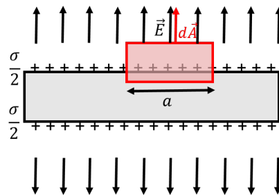
Figure 342: Cross-section of a conducting plane where the charges migrate to the surface. A box-shaped Gaussian surface is also shown as seen from the side (the third dimension of the box is perpendicular to the plane of the page).
