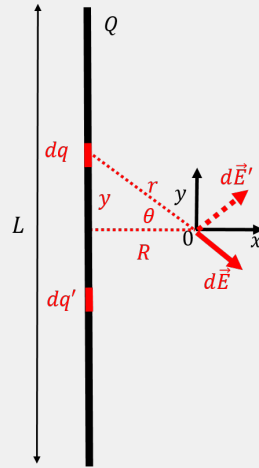
Figure 313: Determining the electric field a distance R from the centre of a rod of length L carrying charge Q .
