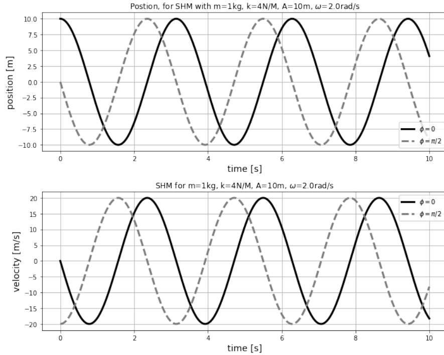
Figure 228: Position and velocity as a function of time for a mass-spring system for two different values of the phase, \phi .
