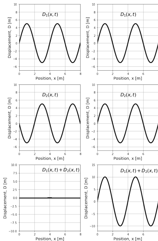
Figure 260: Destructive (left) and constructive (right) interference of waves.
