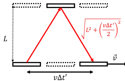
Figure 474: A clock is made by having a pulse of light bounce back and forth between two parallel mirrors separated by a distance, L . When the clock is placed on a spaceship moving with speed, v , the light travels a longer distance before completing a full cycle, as observed by someone not travelling with the clock.
