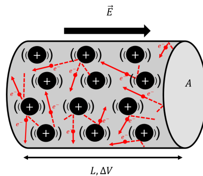
Figure 364: Electrons moving inside a conductor only “drift” on average in the direction anti-parallel to the electric field. In reality, they constantly collide with atoms in the material, transferring their kinetic energy into thermal energy of the conductor.
