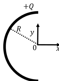
Figure 308: A charged wire bent into a semi-circle of radius R .
