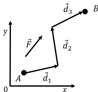
Figure 128: An arbitrary two dimensional path of an object from A to B broken into three straight segments.
