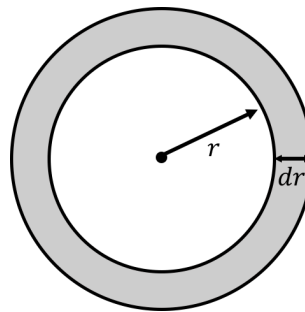
Figure 258: A spherical shell at radial position r with thickness dr
