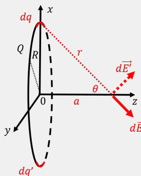
Figure 311: Determining the electric field on the axis of a ring of radius R carrying charge Q .
