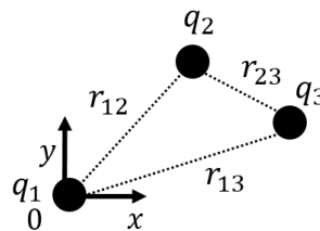
Figure 347: Three positive charges arranged together will store a certain amount of electrostatic potential energy.
