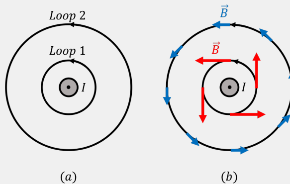
Figure 442: Left: 2 Amperian loops around a current carrying wire. Right: Magnetic field vectors around each loop.
