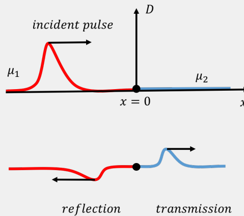
Figure 266: An incident pulse propagates through a rope connected to a another rope with a different linear mass density. When it reaches the boundary, part of the pulse is reflected and part is transmitted. Whether the reflected pulse is inverted or upright will depend on the reflection coefficient.
