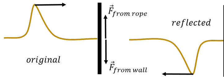
Figure 251: When the end of the rope is held fixed, the reflected pulse will be inverted.
