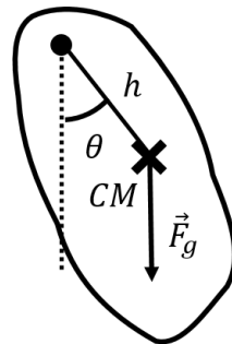
Figure 234: A physical pendulum which oscillates in a vertical plane about an axis through the object.
