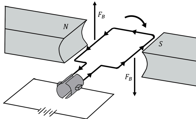
Figure 426: Illustration of a DC electric motor. Current circulates in the coil resulting in a torque from the magnetic field. Once the coil is aligned with the magnetic field, the direction of the current in the coil is inverted, so that the coil continues to feel a torque. The current is inverted using mechanical brushes that reverse the leads on the coil every half turn.
