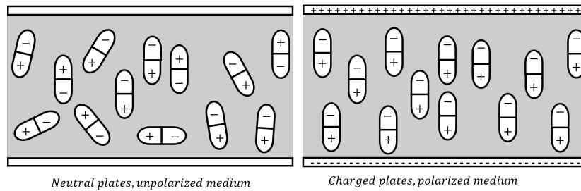
Figure 359: A dielectric material is placed between the two plates of a capacitor. The electric dipoles in the dielectric have random orientations when the plates are neutral (left panel). When the plates are charged (right panel), the dipoles align themselves with the field from the plates, allowing more charge to be on the plates at a given potential difference.
