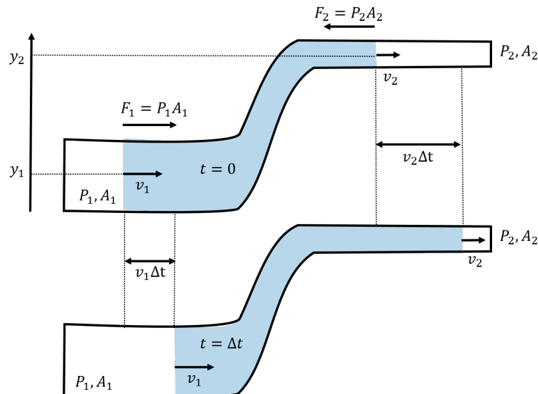
Figure 284: Laminar flow of an incompressible fluid through a pipe that changes cross-sectional area and height in the direction of flow. An element of fluid, in blue, is shown at time t = 0 (top panel), and then, at a later time, t = \Delta t (bottom panel).
