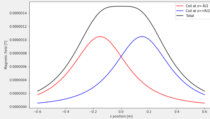
Figure 452: Magnetic field from each coil, as well as their sum, for two coils in the Helmholtz configuration
