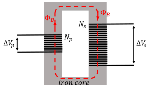
Figure 463: A transformer converts a primary alternating voltage, \Delta V_p , to a secondary alternating voltage, \Delta V_s . The magnetic flux produced in one coil is transmitted by an iron core to the secondary coil, where a different voltage is induced, depending on the ratio of the number of windings in each coil.
