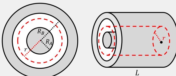
Figure 361: Solving for E between two cylinders using Gauss' law.
