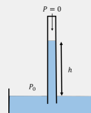
Figure 279: A Torricelli barometer.
