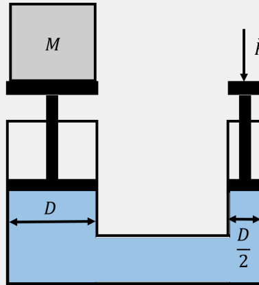
Figure 275: A force exerted on the piston of a hydraulic lift in order to lift a mass M .
