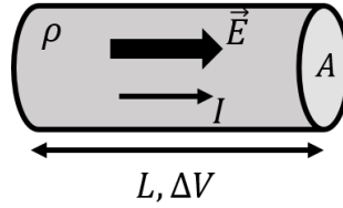
Figure 367: A simple resistor of length, L , cross-sectional area, A , made from a materials with resistivity, \rho . A potential difference, \Delta V , is applied across the resistor, leading to an electric field and current in the resistor.
