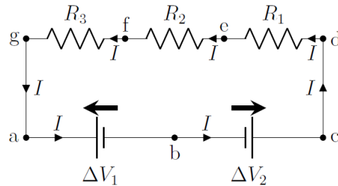
Figure 387: A loop with 2 batteries and 3 resistors.
