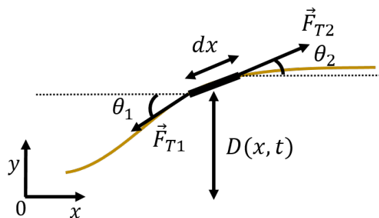
Figure 254: A small section of rope under tension as a wave passes through.
