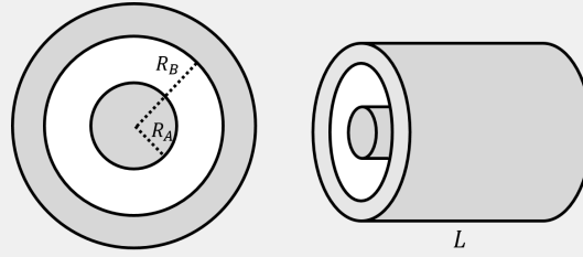
Figure 360: A capacitor constructed from concentric cylinders.
