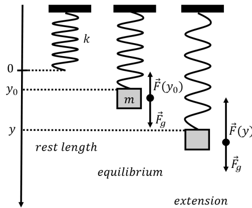
Figure 231: A vertical spring-mass system.
