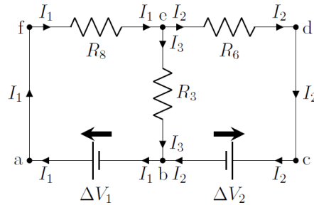
Figure 393: Final and labelled circuit diagram that is simplified from the one in Figure 16 .
