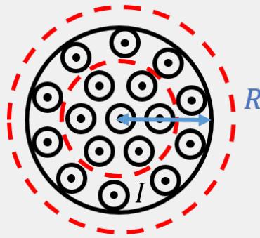
Figure 443: Two circular Amperian loops to determine the magnitude of the magnetic field inside and outside of a current-carrying cable of radius, R (with uniform current coming out of the page).
