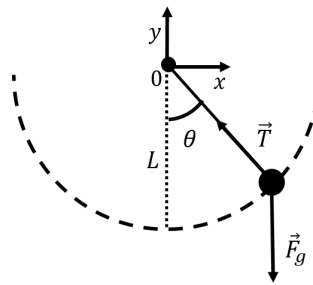
Figure 233: A simple pendulum which oscillates in a vertical plane.
