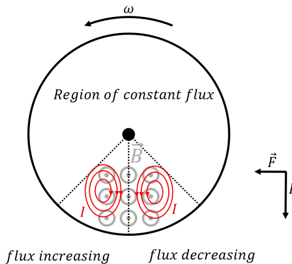
Figure 462: A rotating wheel made of a conducting material has a small region with a magnetic field. The eddy currents in the region of changing flux result in a net downwards current at the centre of the region. The magnetic force that is exerted on that current slows down the wheel.
