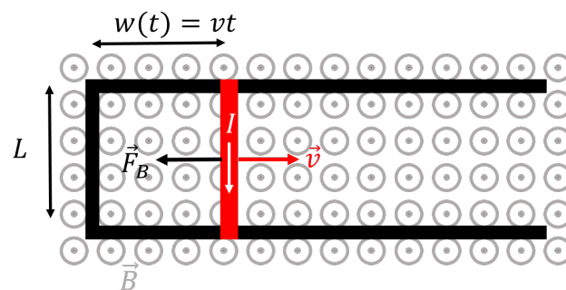
Figure 457: A U-shaped rail on top of which a bar of length, L , can slide. The system is immersed in a magnetic field that points out of the page. The bar moves to the right with a constant speed, v .
