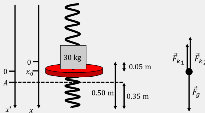
Figure 239: The forces acting on the platform and our new coordinate system.
