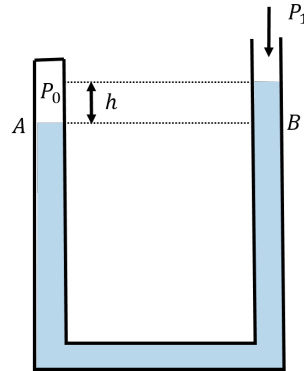
Figure 277: A barometer constructed from a manometer to measure relative changes in atmospheric pressure.
