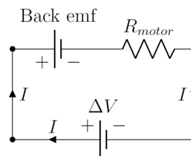
Figure 459: A simple circuit illustrating how a motor, with resistance, R_{motor} , will generate a “back emf”, equivalent to a battery that produces a voltage in the direction to oppose the current from the actual battery that is powering the motor, \Delta V .
