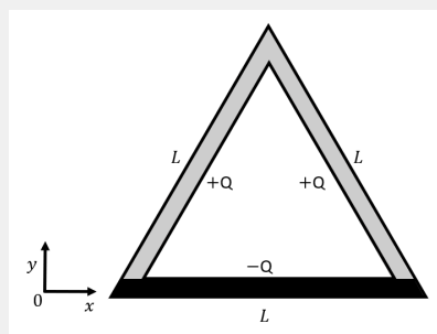
Figure 321: A triangle made up of charged rods
