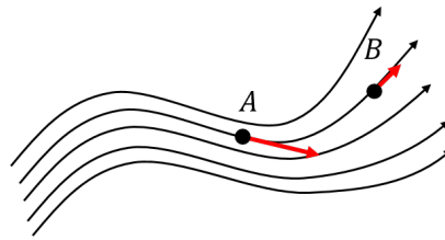
Figure 306: An example of determining a field vector from the continuous field lines.
