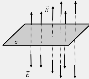
Figure 340: The electric field above an infinite plane with uniform charge per unit area, \sigma , must be perpendicular to the plane.
