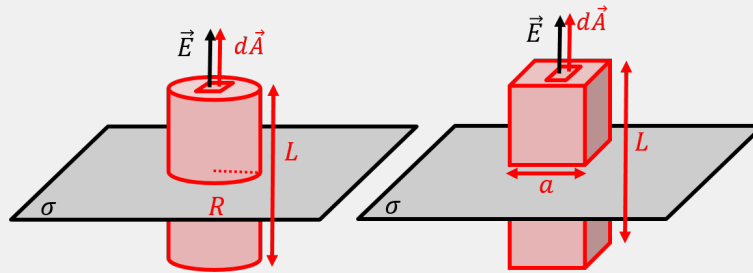
Figure 341: A cylindrical surface or a box are both good choices for a Gaussian surface above a plane, since only the parts of the surface parallel to the plane will have net flux through them.
