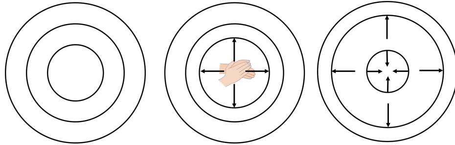
Figure 257: Left: We divide the air into thin spherical shells. Here we represent three shells (the black circles). Center: When you clap, the innermost shell is given energy and expands. Right: Energy is transferred to the next shell, which expands as the first shell contracts. This is how the wave propagates outwards. When the shells are closer together, the air molecules are closer together and exert a pressure that tries to expand the shell.
