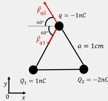
Figure 302: Force vectors on charge q .
