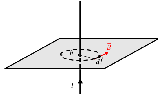
Figure 441: An Amperian loop that is a circle of radius, h , will allow us to determine the magnetic field at a distance, h , from an infinitely-long current-carrying wire.
