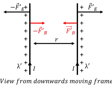
Figure 467: Two infinitely-long charged wires as viewed from a down-going frame of reference will appear to have upwards-going currents that will result in an attractive magnetic force between the wires.
