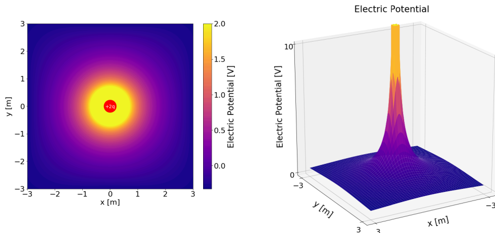
Figure 352: Electric potential heat map (left) and surface plot (right) near a single positive charge.
