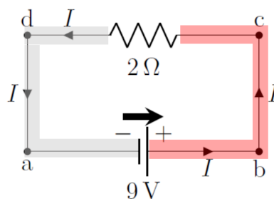
Figure 378: The same circuit as in Figure 4 showing the two regions over which the electric potential is constant.
