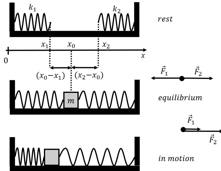
Figure 232: A mass attached to two different springs.
