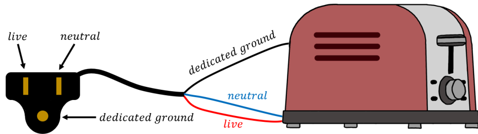
Figure 373: When an appliance has three prongs on its electrical cable, the middle prong grounds the case to the dedicated ground as a safety measure. Note that the live wire is not necessarily the right-hand side socket on an outlet!
