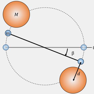
Figure 237: Two very large spheres are placed near each of the small masses on the torsional pendulum (top view). At the new equilibrium, each small mass is a distance d from the nearest large mass.
