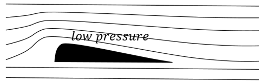
Figure 285: Laminar flow of air around an airfoil. The curvature of the asymmetric airfoil forces the streamlines above the airfoil together, increasing the speed of the air due to the continuity equation, and resulting in a low pressure area.
