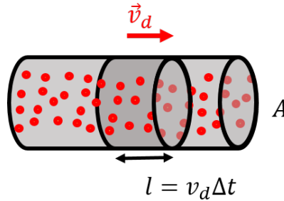
Figure 365: A section of electrons of length l drifting through a conductor of cross-sectional area, A .
