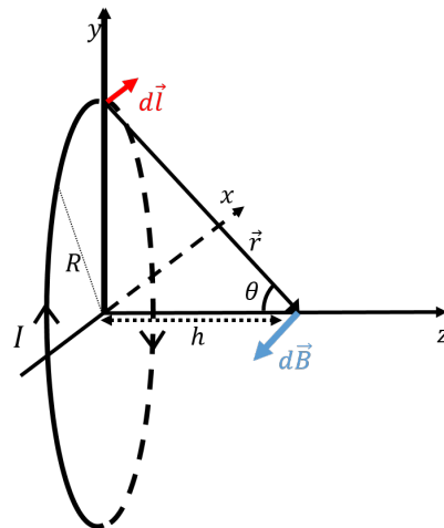
Figure 435: Diagram to apply the Biot-Savart Law in order to determine the magnetic field along the symmetry axis of a ring carrying current, I . The x axis goes into the page.
