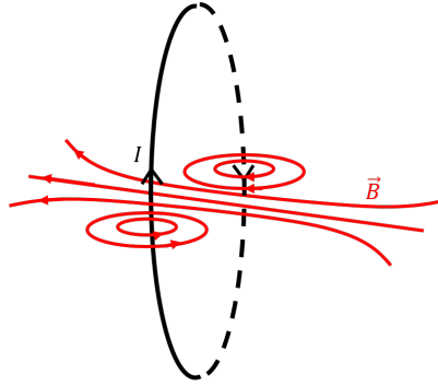
Figure 434: The magnetic field from a current-carrying loop of wire can be thought of as the sum of the fields from small straight sections of wire.
