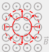
Figure 454: A loop whose radius increases with time.
