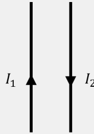
Figure 438: Two wires that carry current in opposite directions.
