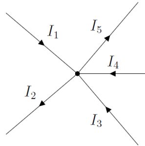
Figure 386: A junction with 5 segments and 5 currents.
