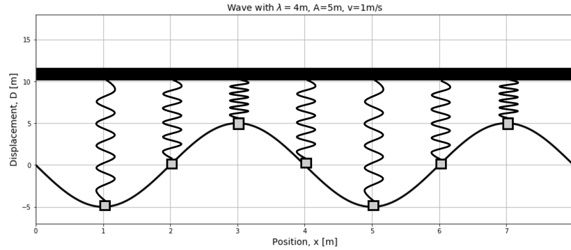
Figure 256: The displacement as a function of position for different points in a medium. Each point in the medium can be modelled as a simple harmonic oscillator.
