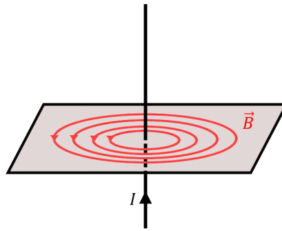
Figure 433: The magnetic field from a current-carrying wire forms concentric circles centred on the wire.
