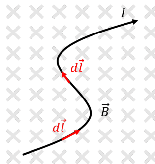
Figure 416: The magnetic force on a curved current-carrying wire is obtained by modelling the forces exerted on infinitesimal sections of wire, each with length d\vec{l} , and summing together those forces to get the total force on the wire.
