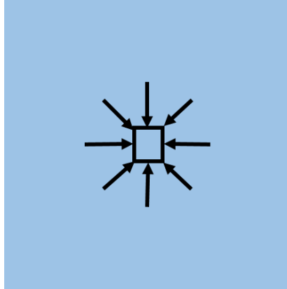
Figure 268: A small element inside of a fluid with pressure will experience no net force from the pressure in the fluid, since the force associated with the pressure in the fluid is exerted in all directions.
