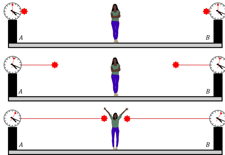
Figure 471: Alice is equidistant from two clocks. The clocks fire a laser pulse when the time is 20 past four, and Alice observes both pulses arriving at her location at the same time, concluding that the pulses were emitted by the clocks at the same time.
