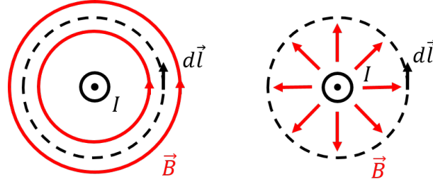
Figure 440: By symmetry, the magnetic field from a current-carrying infinite wire (illustrated with current coming out of the page), must either form concentric circles (left panel), or be in the radial direction (right panel). We know that the former (circles, left panel) is the correct choice. The dotted lines show “Ampèrian loops” that one can use to calculate the integral in Ampère’s Law.
