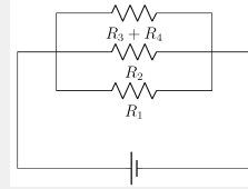
Figure 398: A much less weird looking circuit.
