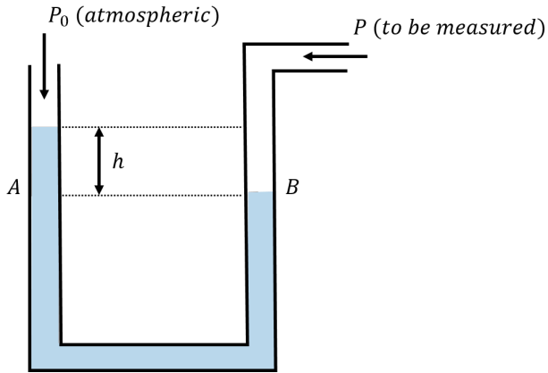
Figure 276: A manometer can measure the difference between a pressure P and atmospheric pressure, P_0 . That difference is called “gauge pressure”.
