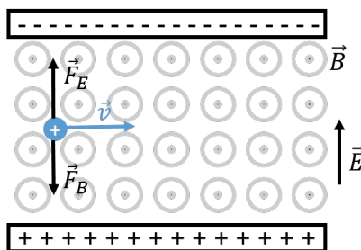
Figure 425: Illustration of a velocity selector. Only charged particles with a specific speed can make it through without colliding with one of the plates.
