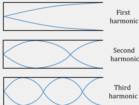
Figure 266: The first three harmonics for a clarinet. There is a node at the fixed end and an anti-node at the free end.
