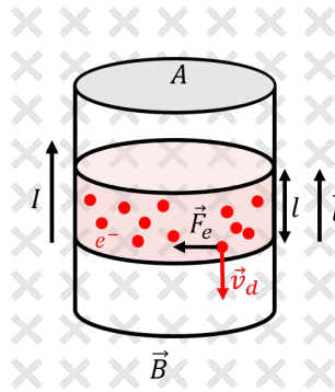
Figure 415: A section of wire carries conventional current, I , upwards while being immersed in a uniform magnetic field, \vec{B} , into the page. We introduce a vector, \vec{l} , to represent a section of wire of length l carrying current in the direction of \vec{l} .
