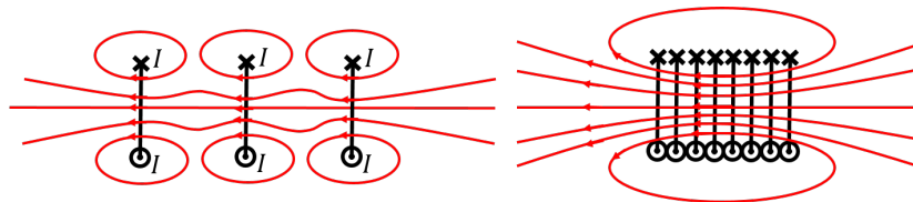
Figure 447: As multiple loops of current are brought together to form a solenoid, the magnetic field inside the solenoid becomes uniform and the field outside the solenoid approaches zero.
