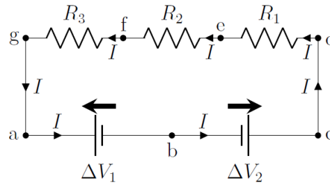
Figure 388: A loop with 2 batteries and 3 resistors.
