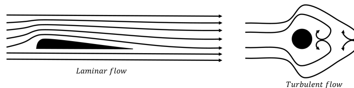
Figure 282: Laminar (left) and turbulent (right) flow of a fluid around an object.
