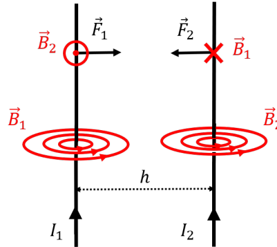
Figure 438: Two parallel current-carrying wires will exert an attractive force on each other, if their currents are in the same direction.
