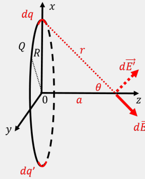
Figure 312: Determining the electric field on the axis of a ring of radius R carrying charge Q .
