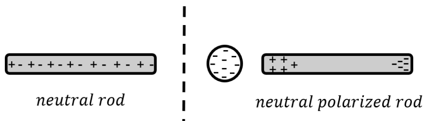
Figure 298: Electrostatic induction: when a negatively charged sphere is brought close to a neutral conducting rod, the electrons in the rod, which can move freely, accumulate on the side of the rod furthest from the sphere, leaving an excess of positive charge near the sphere.
