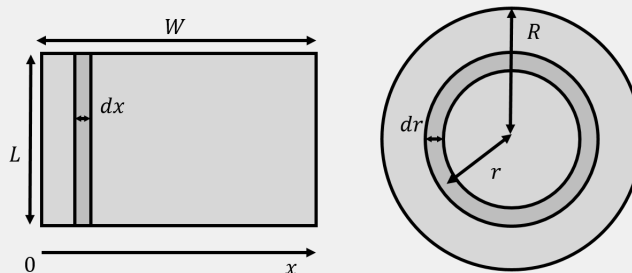
Figure 315: A two-dimensional object such as a plane modelled as a the sum of infinitely thin lines (left panel) or as the sum of infinitely thin rings (right panel).
