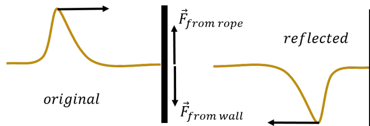
Figure 252: When the end of the rope is held fixed, the reflected pulse will be inverted.
