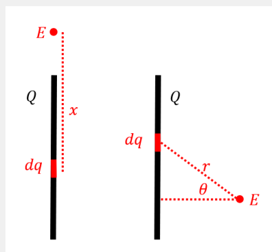
Figure 318: Calculating the electric field produced by a rod at different positions.
