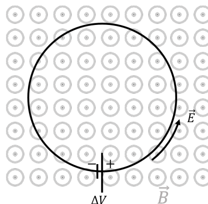
Figure 461: A varying magnetic field will induce a circular electric field.
