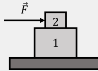
Figure 93: Two stacked boxes.
