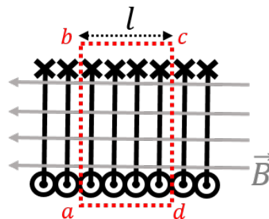
Figure 449: By extending the Amperian loop to both sides of the solenoid, we conclude that the magnetic field just outside the solenoid must be zero, because the net current enclosed is zero.
