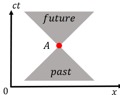
Figure 482: The past and future light cones associated with the space-time event, A .
