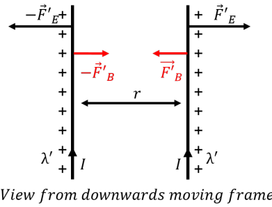
Figure 468: Two infinitely-long charged wires as viewed from a down-going frame of reference will appear to have upwards-going currents that will result in an attractive magnetic force between the wires.
