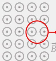
Figure 456: A loop being pulled out of a region with uniform magnetic field.
