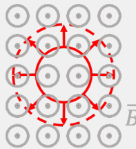
Figure 455: A loop whose radius increases with time.
