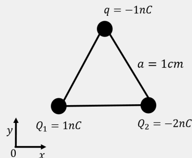
Figure 302: Three charges arranged in an equilateral triangle of side a .
