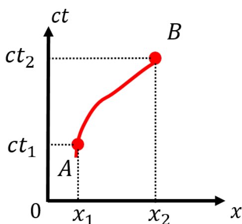
Figure 481: World line of an object that moved from locations A in space-time to location B in space-time.
