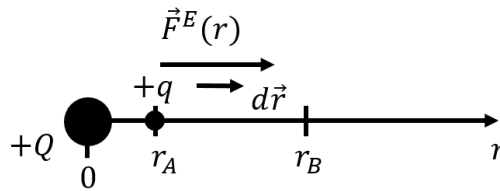
Figure 347: Calculating the work done on a charge +q by the electric force exerted by charge +Q when charge +q moves from a distance r_A to a distance r_B from the centre of charge +Q .
