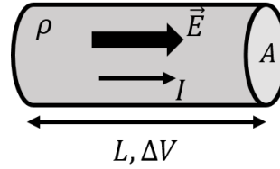
Figure 368: A simple resistor of length, L , cross-sectional area, A , made from a materials with resistivity, \rho . A potential difference, \Delta V , is applied across the resistor, leading to an electric field and current in the resistor.
