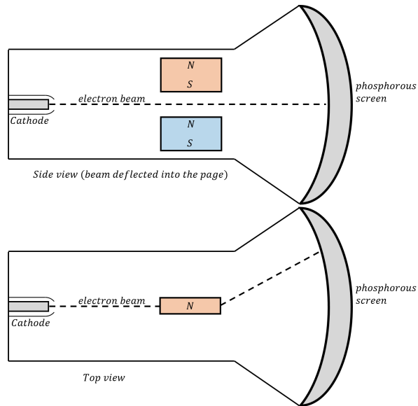
Figure 428: Illustration of a cathode ray tube from a side view (top) and a top view (bottom). A magnetic field is used to deflect a beam of electrons onto a screen. The perpendicular magnetic fields are used to sweep the beam rapidly across the whole screen to create an image.
