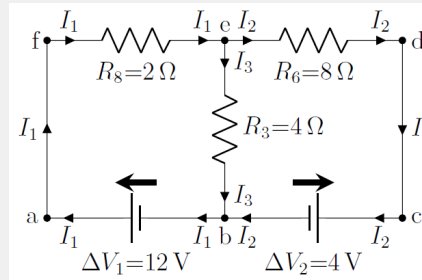
Figure 396: Simplified version of the circuit in Figure 21 .
