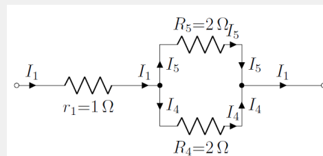
Figure 397: The components of the effective R_8 resistor from Figure 22 . The current, I_1 , coming from the battery goes through r_1 and then splits up.
