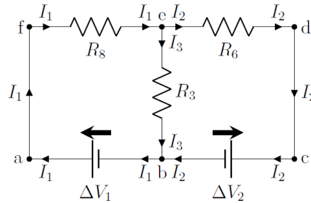
Figure 394: Final and labelled circuit diagram that is simplified from the one in Figure 16 .
