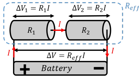
Figure 369: When two resistors are connected in series, the same current flows through each resistor.
