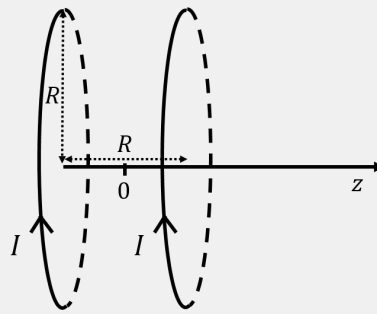
Figure 452: A Helmholtz coil arrangement.
