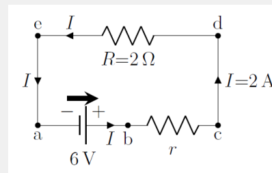
Figure 384: A circuit showing a real battery (with internal resistance r ) in series with a resistor.
