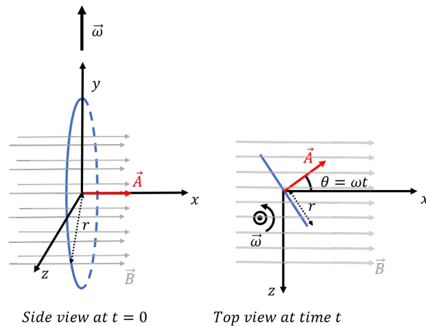
Figure 459: A loop of wire rotates in a constant and uniform magnetic field. At time t = 0 (left panel), the loop lies in the yz plane. The loop rotates about the y axis, with a constant angular velocity, \vec{\omega} . At some time t later, the loop has rotated through an angle \theta = \omega t (right panel, as seen from above, looking down on the xz plane).
