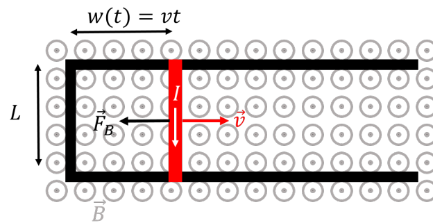
Figure 458: A U-shaped rail on top of which a bar of length, L , can slide. The system is immersed in a magnetic field that points out of the page. The bar moves to the right with a constant speed, v .
