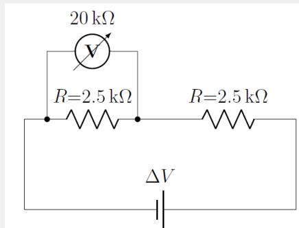
Figure 408: A circuit with a battery of unknown voltage.
