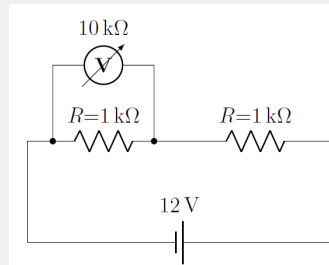
Figure 405: When using a voltmeter, the circuit is modified.
