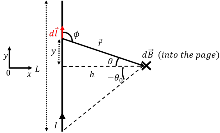
Figure 433: Setting up the model to use the Biot-Savart Law to calculate the magnetic field a distance h from the centre of a current-carrying wire of length L .
