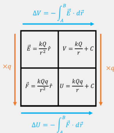
Figure 351: How you would use the guide in the case of a point charge, Q , exerting a force on another point charge, q .
