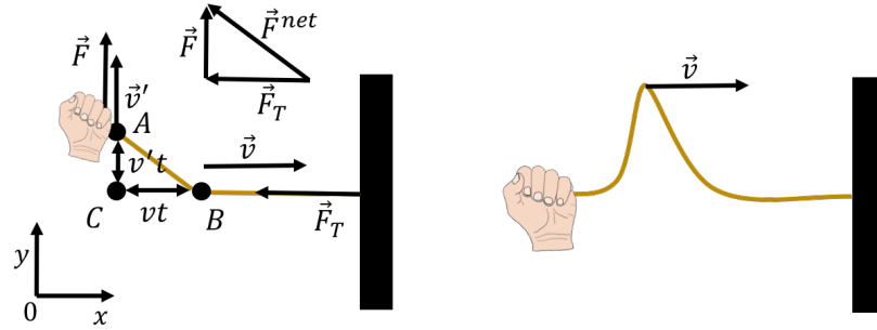
Figure 251: (Left:) Pulling upwards and then downwards on a horizontal rope causes a pulse to form and propagate. After a short period of time, a pulse is seen propagating down the rope (right).
