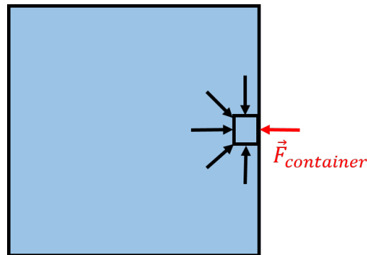
Figure 270: At the edge of a container, a small element of fluid will exert an outwards force on the container, and the container will exert an inwards force on the element of fluid.
