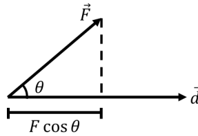
Figure 122: When determining the scalar product \vec{F} \cdot \vec{d} = Fd \cos \theta , \theta is the angle between the vectors when they are placed tail to tail.
