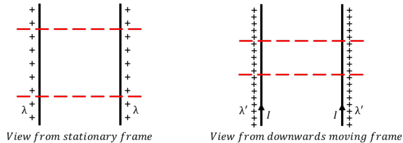
Figure 469: Two infinitely-long charged wires as viewed from a rest frame and a moving frame. In order for the charge density to be greater in the moving reference frame, the wire must be shorter. For an infinitely long wire, this is depicted by
