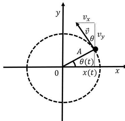
Figure 230: Uniform circular motion of a particle along a circle of radius A with constant angular speed \omega .
