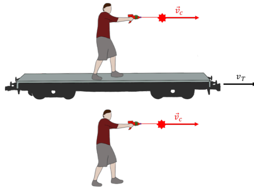
Figure 471: Two people fire a laser pulse. Regardless of whether the pulse of laser light was fired from a moving train or from the ground, it will have a speed of c in all frames of reference.
