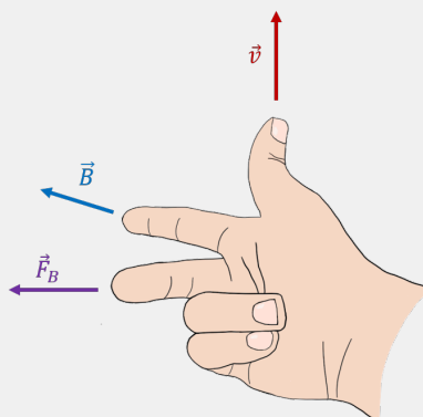
Figure 412: The way that Josh remembers the right hand rule for magnetism.
