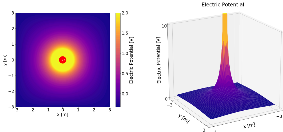
Figure 353: Electric potential heat map (left) and surface plot (right) near a single positive charge.
