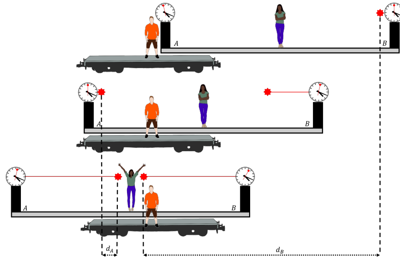
Figure 473: Brice is on a moving train, and, from his perspective, it is Alice and the platform that are moving towards him. Brice must conclude that the pulse from clock B was emitted earlier, since it must travel further than the pulse emitted from clock A to reach Alice at the same time.
