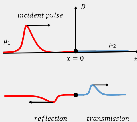
Figure 267: An incident pulse propagates through a rope connected to a another rope with a different linear mass density. When it reaches the boundary, part of the pulse is reflected and part is transmitted. Whether the reflected pulse is inverted or upright will depend on the reflection coefficient.
