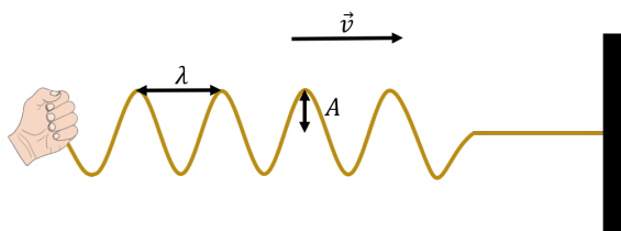
Figure 248: Wavelength, velocity, and amplitude for a transverse wave on a rope.
