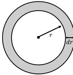
Figure 259: A spherical shell at radial position r with thickness dr
