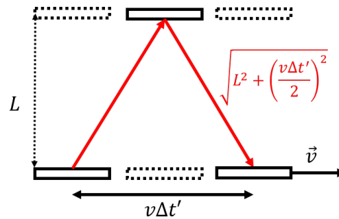
Figure 475: A clock is made by having a pulse of light bounce back and forth between two parallel mirrors separated by a distance, L . When the clock is placed on a spaceship moving with speed, v , the light travels a longer distance before completing a full cycle, as observed by someone not travelling with the clock.
