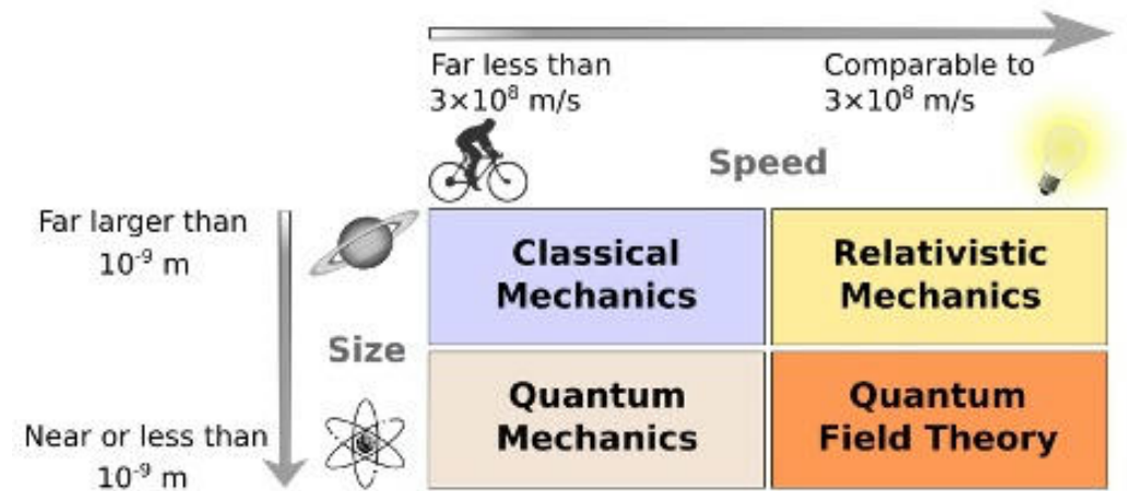
Figure 3: Classical mechanics works for larger and slower objects; modern theories are needed otherwise. Credit: Yassine Mrabet.
