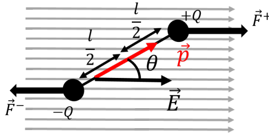
Figure 321: An electric dipole in a uniform electric field.
