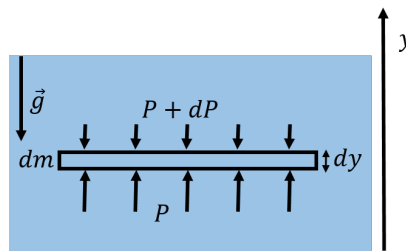
Figure 273: Pressure gradient from gravity on an infinitesimal fluid element.
