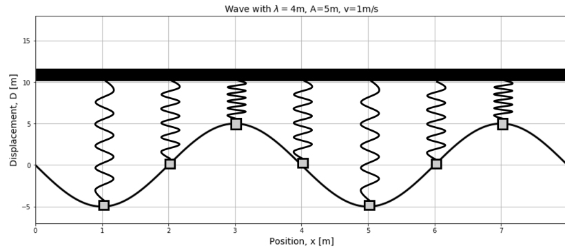
Figure 257: The displacement as a function of position for different points in a medium. Each point in the medium can be modelled as a simple harmonic oscillator.
