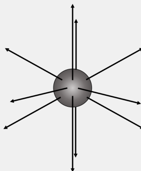
Figure 332: The field lines for a positively charged sphere.
