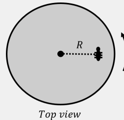
Figure 117: An ant on a horizontal turntable that is starting to spin, as seen from above.
