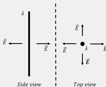
Figure 336: An infinite line of charge carrying uniform charge per unit length, \lambda . The left panel shows a side view and the right panel a view from above. The electric field must be in the radial direction or there would be a preferred direction.
