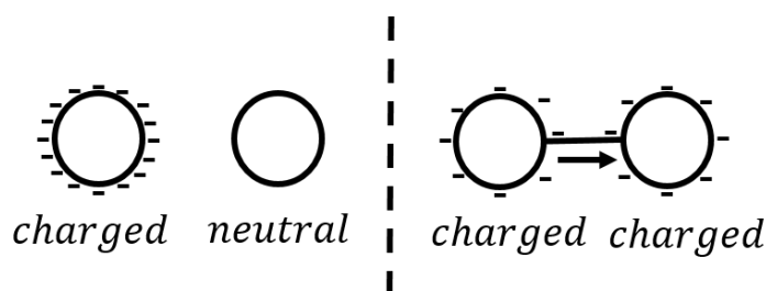
Figure 297: Charging by conduction: a neutral conducting sphere is connected to a negatively charged conducting sphere. The charges can “spread out more” if some of the charges move (“conduct”) from the charge sphere onto the neutral sphere.
