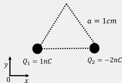
Figure 304: Two charges at the corners of an equilateral triangle of side a .
