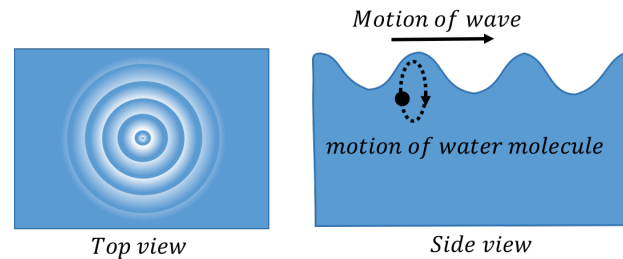
Figure 243: A transverse wave travelling through water. The left panel shows the view from above as ripples move outwards. The right panel shows the motion of an individual water molecule as the wave is viewed from the side.
