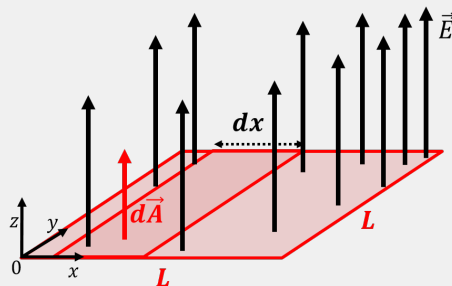
Figure 326: Dividing a square in the xy plane into thin strips of length L and width dx .
