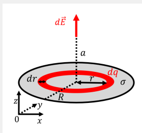
Figure 316: Modelling the field from a disk as the sum of fields from concentric thin rings.
