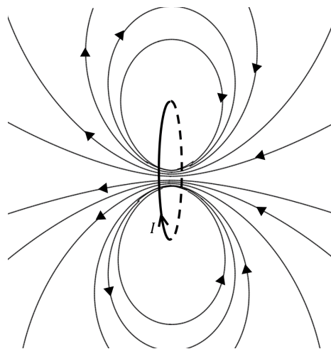
Figure 411: The magnetic field lines produced by a circular loop of current, I , are the same as those produced by a bar magnet.
