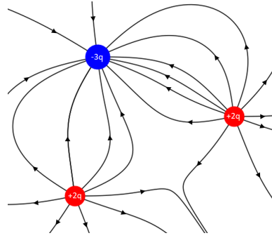
Figure 308: Field lines of two +2q charges and one -3q charge.
