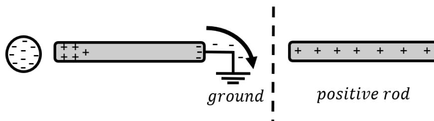
Figure 299: Charging by induction: when we connect the polarized rod to the ground, electrons can leave the rod. If we now disconnect the rod from ground, the rod is left with an overall positive charge.
