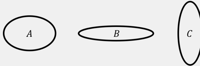
Figure 170: Three ellipses, each with a different eccentricity.
