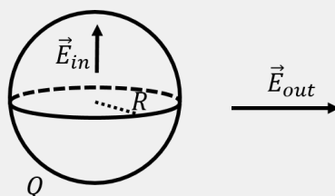
Figure 329: For a spherical charge distribution, the electric field inside and outside must point in the radial direction, by symmetry.
