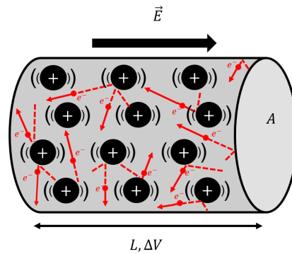
Figure 365: Electrons moving inside a conductor only “drift” on average in the direction anti-parallel to the electric field. In reality, they constantly collide with atoms in the material, transferring their kinetic energy into thermal energy of the conductor.
