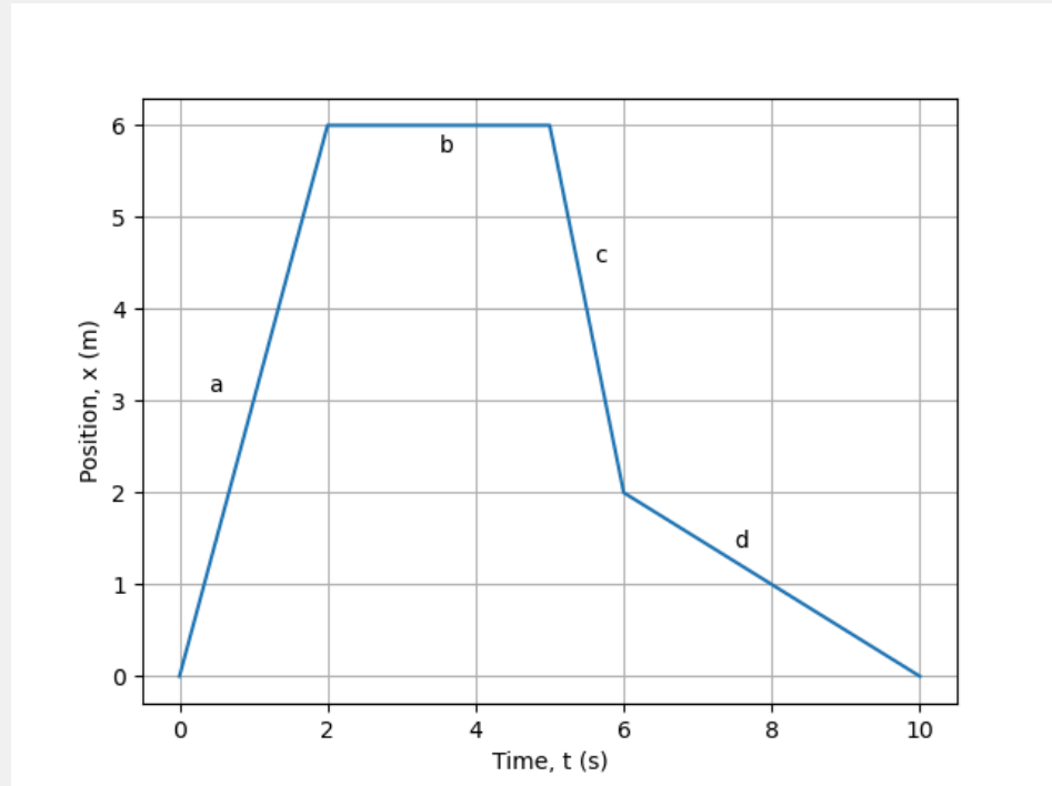
Figure 38: Plot of position as a function of time for an object moving at varying velocities, labeled a, b, c, d.
