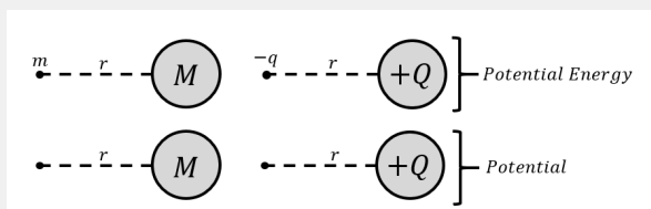
Figure 349: Gravitational potential energy and gravitational potential (left) next to its electrical analogue (right).
