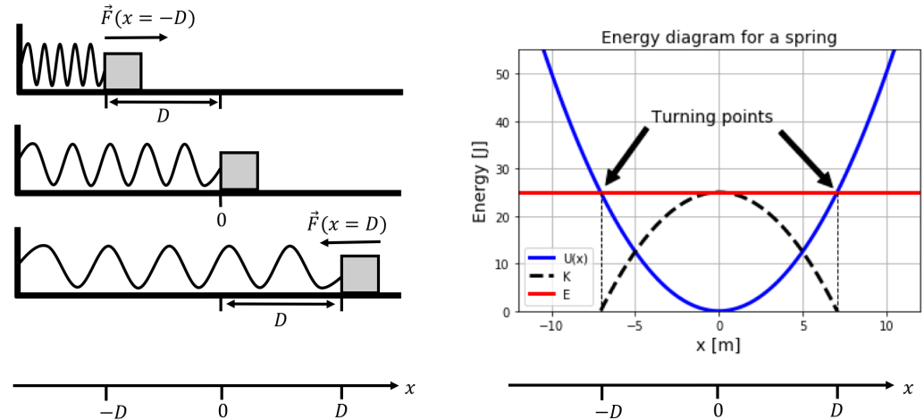
Figure 161: Left: The block oscillates about the rest position of the spring, between x = -D and x = D . Right: The energy diagram for the block. This diagram is for a spring with spring constant k = 1 upright N/m .
