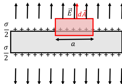
Figure 343: Cross-section of a conducting plane where the charges migrate to the surface. A box-shaped Gaussian surface is also shown as seen from the side (the third dimension of the box is perpendicular to the plane of the page).
