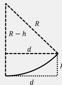
Figure 430: Deflection of an electron moving in a uniform magnetic field.
