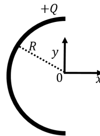
Figure 309: A charged wire bent into a semi-circle of radius R .
