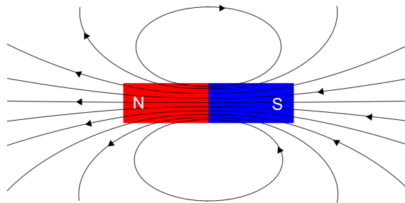
Figure 410: The magnetic field lines for a bar magnet always form closed loops as they do not end at the North or South pole of the magnet.
