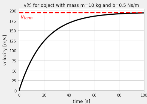
Figure 106: Velocity as a function of time for an object of mass m = upright 10\text{kg} which is free-falling from rest with a drag coefficient b = upright 0.5\text{Ns/m} .
