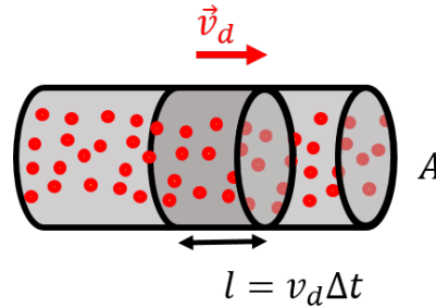
Figure 366: A section of electrons of length l drifting through a conductor of cross-sectional area, A .
