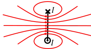
Figure 446: The magnetic field from a single loop of current.
