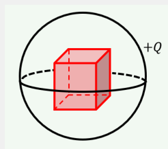
Figure 335: A charged spherical shell with a cubic device inside of it.
