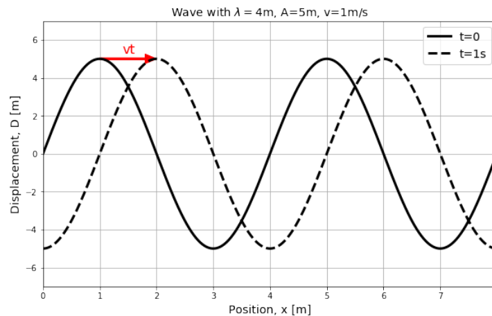
Figure 250: Displacement as a function of position for particles in a medium as a wave passes through. The dotted line shows the displacement as a function of time upright 1/s after the solid line, and corresponds to a wave travelling towards the right.
