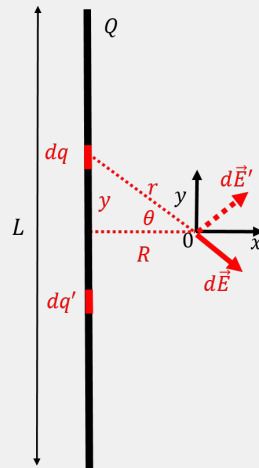
Figure 314: Determining the electric field a distance R from the centre of a rod of length L carrying charge Q .
