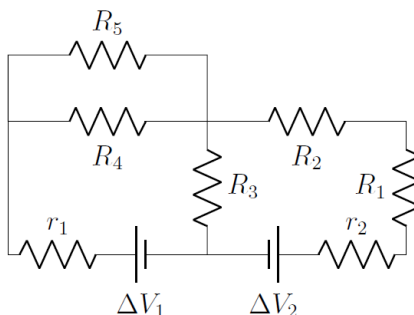
Figure 390: A circuit that can be simplified and then solved with Kirchhoff's rules.
