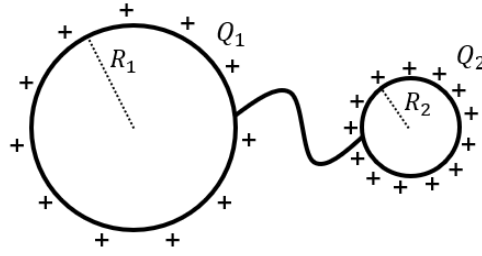
Figure 357: Two conducting spheres are connected by a conducting wire. The charge Q that was originally on the larger sphere distributes itself onto the two spheres.
