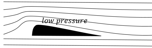
Figure 286: Laminar flow of air around an airfoil. The curvature of the asymmetric airfoil forces the streamlines above the airfoil together, increasing the speed of the air due to the continuity equation, and resulting in a low pressure area.
