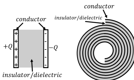
Figure 359: Two examples of capacitors. The left panel shows a “parallel plate” capacitor, and the right panel shows a cylindrically shaped capacitor obtained by “rolling up” a parallel plate capacitor.
