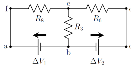
Figure 393: The resistors r_1 and R_7 from the circuit in Figure 18 have been combined into an effective resistor, R_8 , to simplify the circuit.
