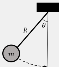
Figure 123: A pendulum swings through an angle \theta .
