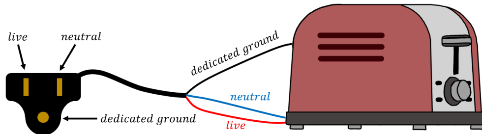
Figure 373: When an appliance has three prongs on its electrical cable, the middle prong grounds the case to the dedicated ground as a safety measure. Note that the live wire is not necessarily the right-hand side socket on an outlet!
