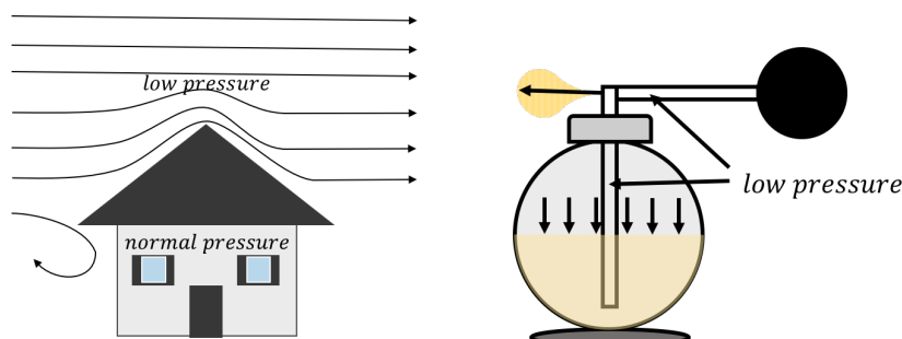
Figure 286: (Left:) the wind flowing above a roof creates a low pressure zone above the roof. (Right:) air flowing above a vertical spout in the atomizer creates a low pressure zone; the air pressure in the bottle forces the liquid up the spout.
