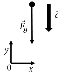
Figure 87: Free-body diagram for a mass that is free-falling in the absence of air resistance (drag).
