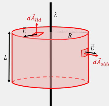
Figure 336: A cylindrical Gaussian surface is used to calculate the flux from an infinite line of charge.
