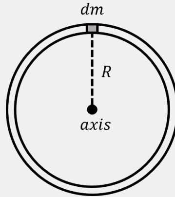
Figure 202: A small mass element on a ring.
