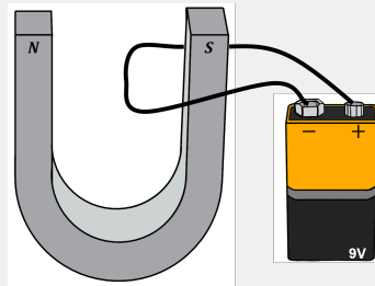
Figure 415: A current carrying wire moving through a magnetic field.
