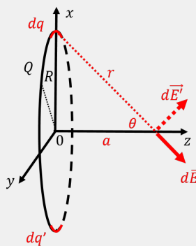
Figure 311: Determining the electric field on the axis of a ring of radius R carrying charge Q .
