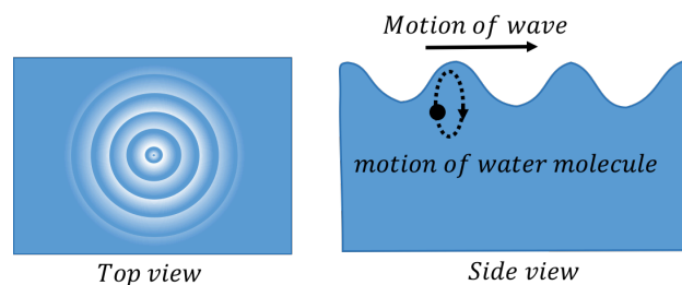
Figure 242: A transverse wave travelling through water. The left panel shows the view from above as ripples move outwards. The right panel shows the motion of an individual water molecule as the wave is viewed from the side.
