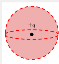
Figure 338: . A spherical Gaussian surface to enclose a point charge.
