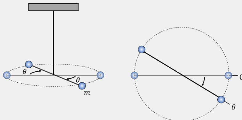
Figure 237: A torsional pendulum. The right side shows a top view.
