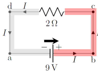
Figure 381: The same circuit as in Figure 4 showing the two regions over which the electric potential is constant.
