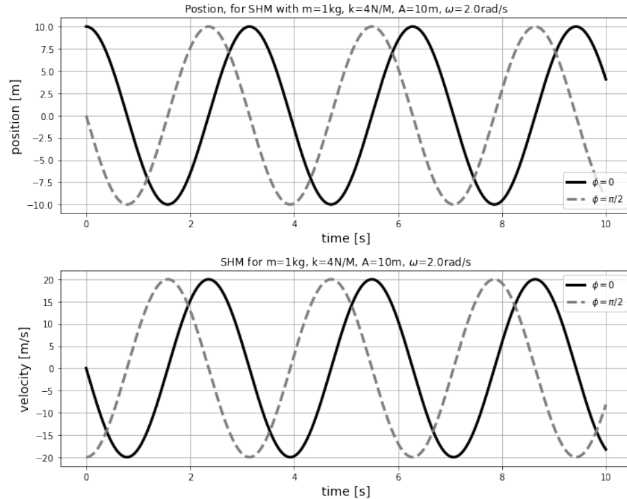
Figure 229: Position and velocity as a function of time for a mass-spring system for two different values of the phase, \phi .
