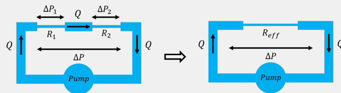
Figure 372: Left panel: What a series circuit would look like in the context of fluid mechanics. Right panel: The two resistors can be thought of as a single resistor with effective resistance R_{eff} = R_1 + R_2 .
