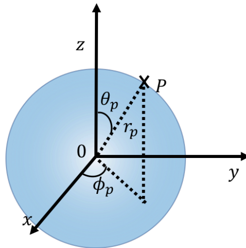
Figure 15: Describing the position of P , located on the surface of a sphere, in spherical coordinates.
