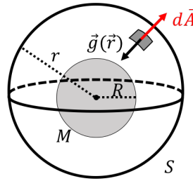
Figure 176: Example of a spherical Gaussian surface, S , of radius r centred about a body of mass M and radius R . An element of the surface, d\vec{A} is also shown along with the gravitational field, \vec{g}(\vec{r}) , at that point.
