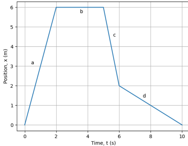
Figure 38: Plot of position as a function of time for an object moving at varying velocities, labeled a, b, c, d.
