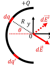
Figure 312: Infinitesimal electric fields from point charges along the bent wire.
