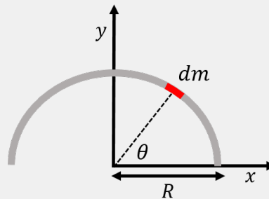
Figure 66: A uniform wire bent into a semi circle of radius R , and a small mass element, dm , on the wire.
