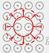
Figure 457: A loop whose radius increases with time.
