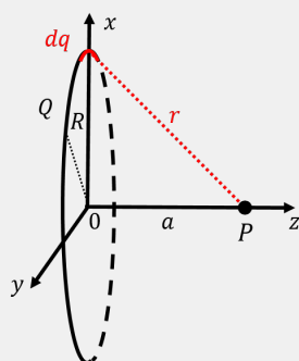
Figure 357: Determining the electric potential on the axis of a ring of radius R carrying charge Q .
