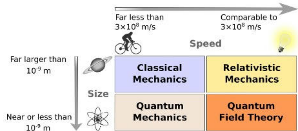
Figure 3: Classical mechanics works for larger and slower objects; modern theories are needed otherwise. Credit: Yassine Mrabet.
