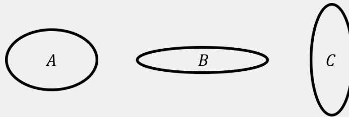
Figure 170: Three ellipses, each with a different eccentricity.
