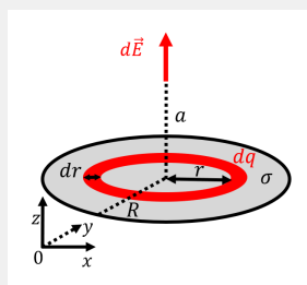
Figure 318: Modelling the field from a disk as the sum of fields from concentric thin rings.
