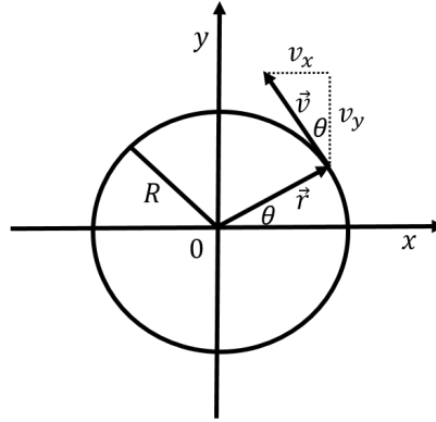
Figure 61: The position vector, \vec{r}(t) is always perpendicular to the velocity vector, \vec{v}(t) , for motion on a circle.
