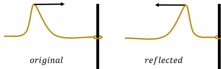
Figure 255: When the end of the rope is free, the reflected pulse will be upright.
