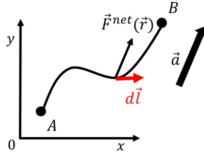
Figure 138: An object moving along an arbitrary path between points A and B that is acted upon by a net force \vec{F}^{net} .
