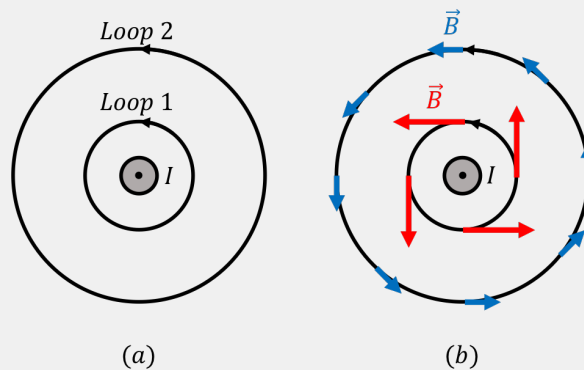
Figure 445: Left: 2 Amperian loops around a current carrying wire. Right: Magnetic field vectors around each loop.
