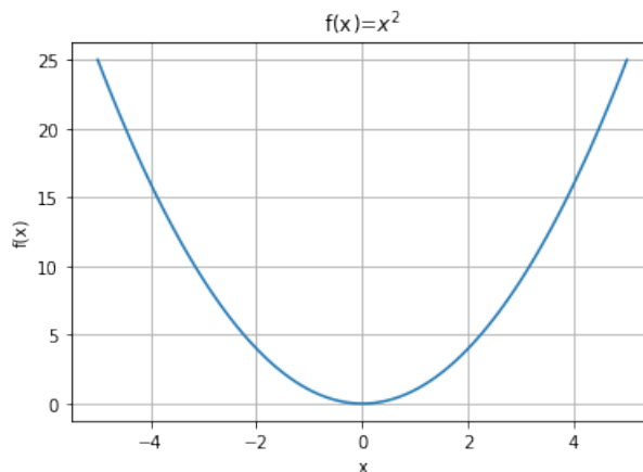
Figure A: f(x) = x^2 plotted between x = -5 and x = +5 .
