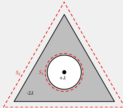
Figure 348: Cross section of the wire/conducting shell set up, showing the Gaussian surfaces.
