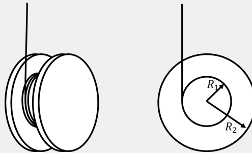
Figure 224: Left: Side view of the yo-yo. Right: Front view of the yo-yo, modelled as two disks of radius of R_2 attached to either side of a disk of radius R_1 .
