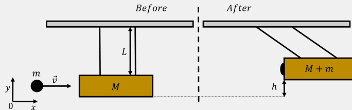
Figure 64: A bullet of mass m strikes and embeds itself into a ballistic pendulum of mass M .
