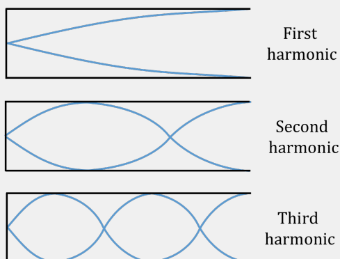
Figure 268: The first three harmonics for a clarinet. There is a node at the fixed end and an anti-node at the free end.
