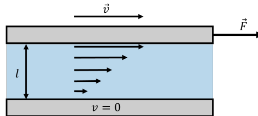
Figure 292: A fluid placed between a moving plate (top) and a fixed plate (bottom) in order to measure the viscosity of the fluid.
