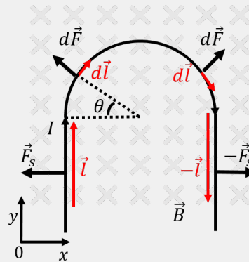
Figure 421: The magnetic force on different sections of wire.
