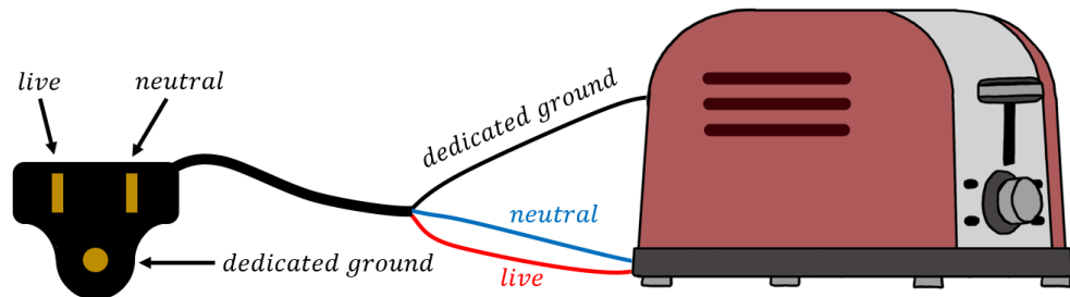
Figure 376: When an appliance has three prongs on its electrical cable, the middle prong grounds the case to the dedicated ground as a safety measure. Note that the live wire is not necessarily the right-hand side socket on an outlet!
