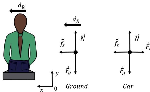
Figure 116: (Left:) A person sitting on a car seat in a car turning towards the left. (Centre:) Free-body diagram for the person as modelled in the inertial reference frame of the ground. (Right:) Free-body diagram for the person as modelled in the non-inertial frame of reference of the car, including an additional inertial force.
