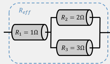
Figure 375: A combination of three resistors.
