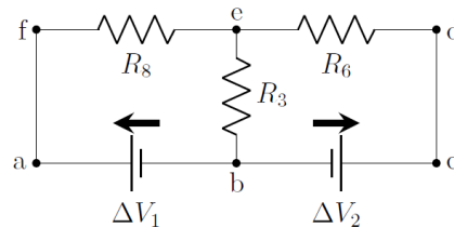
Figure 395: The resistors r_1 and R_7 from the circuit in Figure 18 have been combined into an effective resistor, R_8 , to simplify the circuit.
