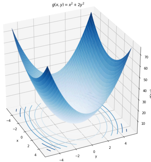
Figure B: g(x, y) = x^2 + 2y^2 plotted for x between -5 and +5 and for y between -5 and +5 . A function of two variables can be visualized as a surface in three dimensions. One can also visualize the function by look at its “contours” (the lines drawn in the xy plane).
