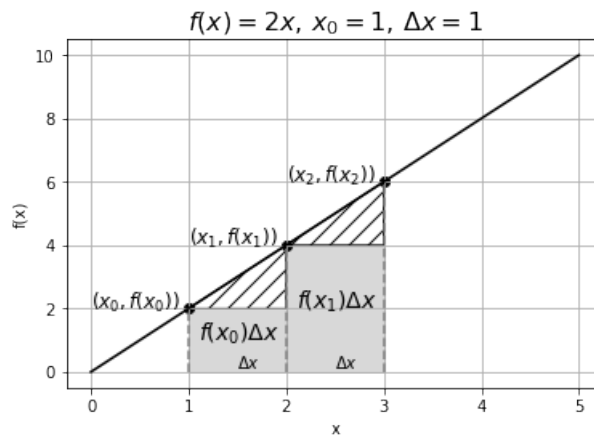
Figure F: The function f(x) = 2x and illustration of the terms f(x_0)\Delta x and f(x_1)\Delta x as the area between the curve f(x) and the x axis when \Delta x \rightarrow 0 .
