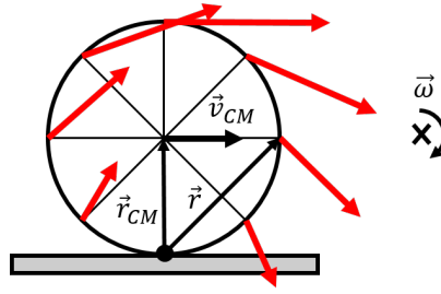
Figure 217: A wheel that is rolling without slipping, as viewed if rotating about the instantaneous axis of rotation that passes through the point of contact with the ground.
