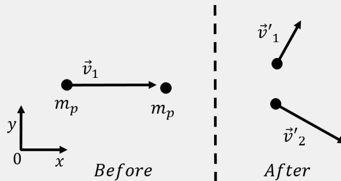
Figure 48: A proton elastically collides with a proton at rest.
