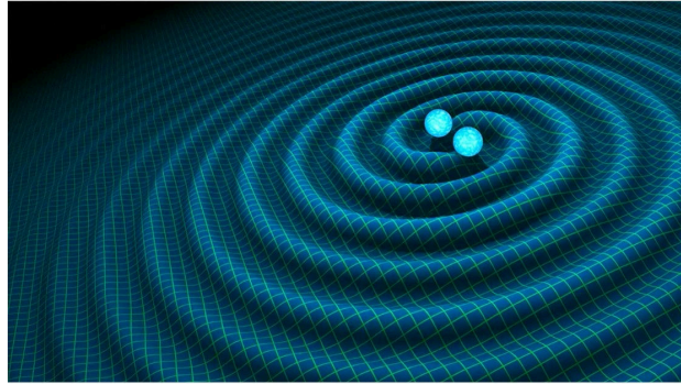
Figure 1: An artist's impression of gravitational waves generated by binary neutron stars. Credit: R. Hurt/Caltech-JPL
