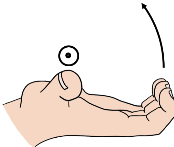
Figure 29: Using the right hand rule for axial quantities. In this case, the direction of rotation is counter clockwise when looking at the page (the direction that the fingers curl), so the rotation vector points out of the page (the direction of the thumb).
