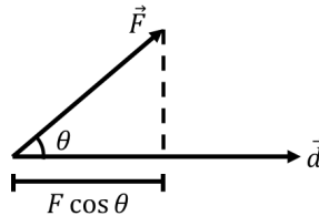
Figure 122: When determining the scalar product \vec{F} \cdot \vec{d} = Fd \cos \theta , \theta is the angle between the vectors when they are placed tail to tail.
