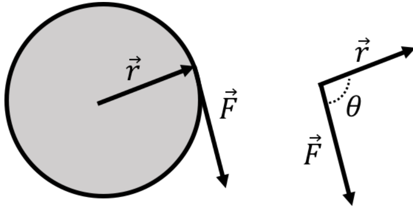
Figure 31: A force, \vec{F} , is exerted in the plane of a disk at a position given by the vector \vec{r} relative to the centre of the disk.
