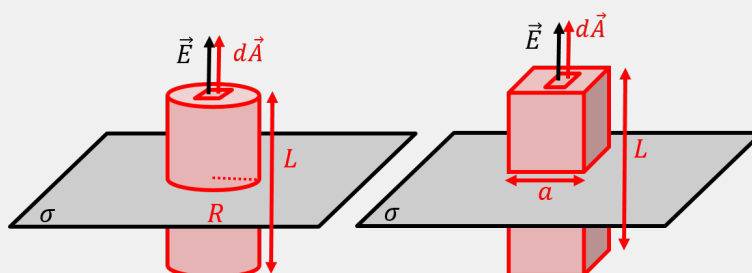
Figure 344: A cylindrical surface or a box are both good choices for a Gaussian surface above a plane, since only the parts of the surface parallel to the plane will have net flux through them.
