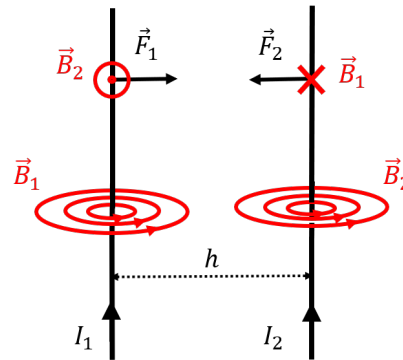
Figure 440: Two parallel current-carrying wires will exert an attractive force on each other, if their currents are in the same direction.
