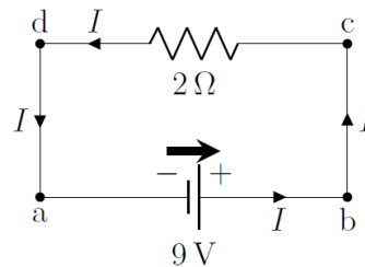
Figure 380: A simple circuit, showing a 9 upright V battery and a 2 upright \Omega resistor. For ease in analyzing circuits, we suggest drawing a “battery arrow” above batteries that goes from the negative to the positive terminal.
