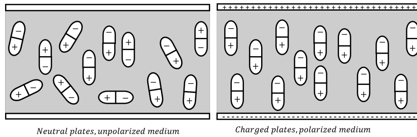
Figure 362: A dielectric material is placed between the two plates of a capacitor. The electric dipoles in the dielectric have random orientations when the plates are neutral (left panel). When the plates are charged (right panel), the dipoles align themselves with the field from the plates, allowing more charge to be on the plates at a given potential difference.
