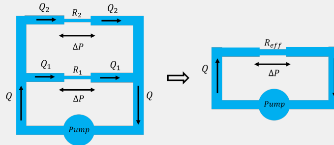
Figure 374: Left panel: What a parallel circuit would look like in the context of fluid mechanics. Right panel: The two resistors can be thought of as a single, wide resistor with effective resistance R_{eff} = (1/R_1) + (1/R_2) .
