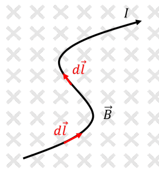
Figure 419: The magnetic force on a curved current-carrying wire is obtained by modelling the forces exerted on infinitesimal sections of wire, each with length d\vec{l} , and summing together those forces to get the total force on the wire.
