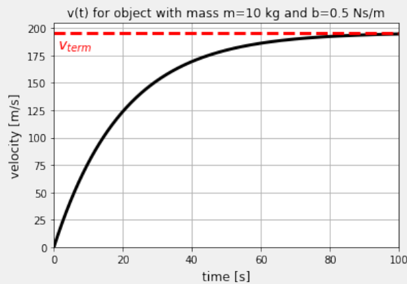
Figure 106: Velocity as a function of time for an object of mass m = upright 10kg which is free-falling from rest with a drag coefficient b = upright 0.5Ns/m .
