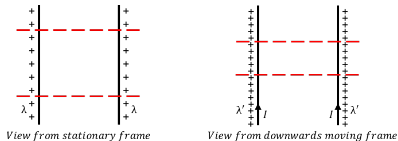
Figure 471: Two infinitely-long charged wires as viewed from a rest frame and a moving frame. In order for the charge density to be greater in the moving reference frame, the wire must be shorter. For an infinitely long wire, this is depicted by
