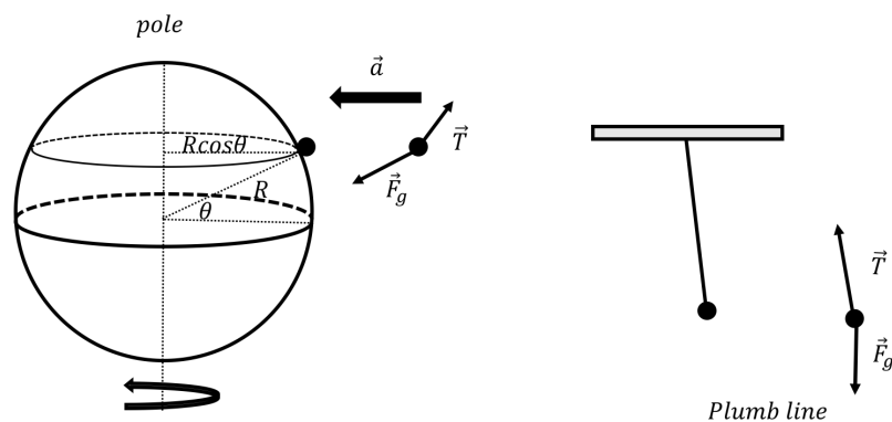
Figure 174: Away from the equator and poles, a plumb line (right) does not point towards the centre of the Earth, because the net force on the mass must provide the acceleration towards the centre of the circle (of radius R \cos \theta ) about which the plumb line rotates due to the Earth's rotation. Note that the deflection of the plumb line is highly exaggerated.
