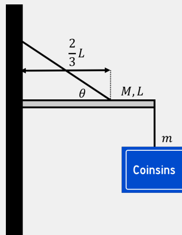
Figure 209: sign is suspended on a horizontal bar of mass M and length L .
