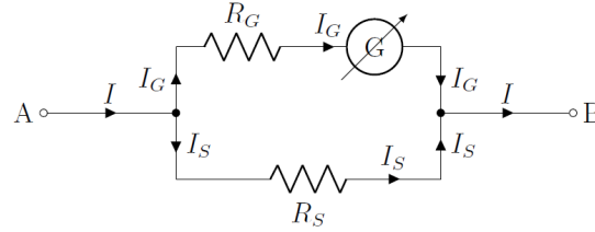
Figure 403: Constructing an ammeter from a galvanometer by placing a “shunt” resistor in parallel with the galvanometer.
