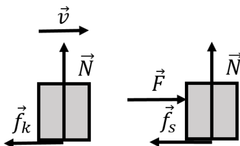
Figure 70: (Left:) A block sliding to the right on a horizontal surface (not shown). The force of kinetic friction, \vec{f}_k , is always perpendicular to the normal force and opposite of the direction of motion. (Right:) A block that is being acted upon by an external force \vec{F} to the right. A force of static friction, \vec{f}_s , is perpendicular to the normal force and opposite the direction of “impeding motion” - without the force of static friction, the block would start to accelerate towards the right, so the force of static friction is to the left.
