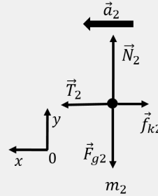
Figure 86: Free-body diagram for m_2 .
