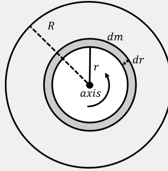
Figure 210: A mass element, dm , in the shape of a ring of radius r and radial thickness dr .
