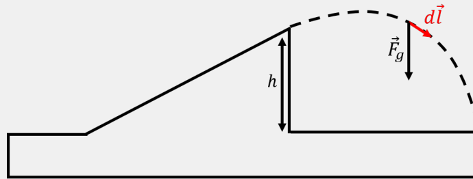
Figure 148: Infinitesimal displacement along the trajectory of the jump.
