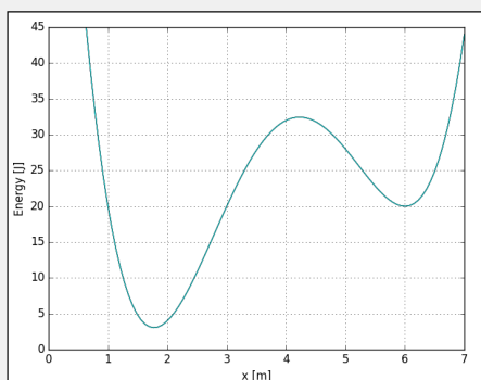
Figure 163: A potential energy function U(x) . The x -axis represents the x position and the y -axis represents the energy.
