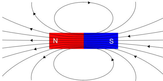
Figure 412: The magnetic field lines for a bar magnet always form closed loops as they do not end at the North or South pole of the magnet.
