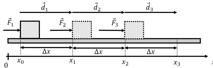
Figure 125: A varying force, \vec{F}(x) , exerted on an object as it moves from position x = x_0 to position x = x_3 .
