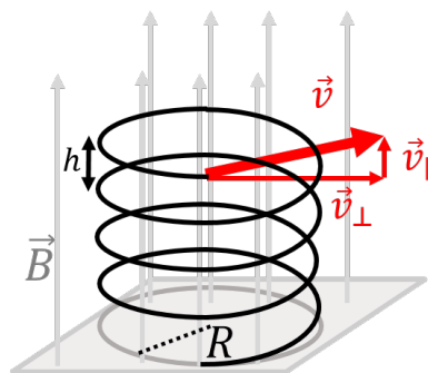
Figure 416: The helical motion of a charged particle with a component of velocity parallel to the magnetic field. The distance, h , between spirals is called the “pitch”.
