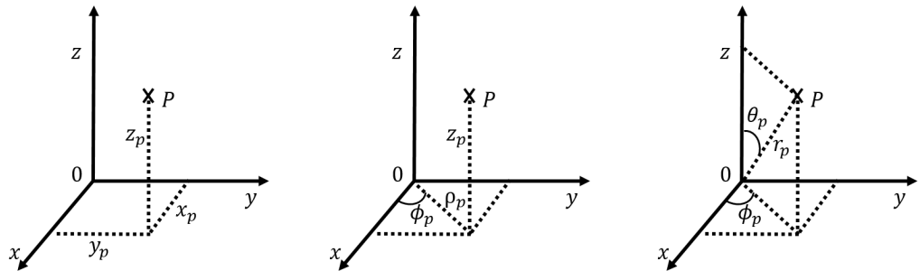
Figure 13: Cartesian (left), cylindrical (centre) and spherical (right) coordinate systems used in three dimensions. The y and z axes are in the plane of the page, whereas the x axis comes out of the page.
