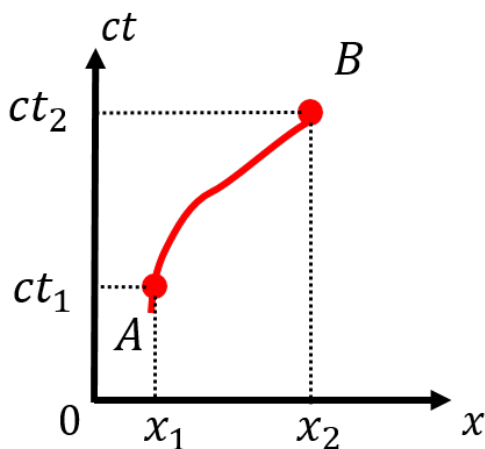
Figure 483: World line of an object that moved from locations A in space-time to location B in space-time.
