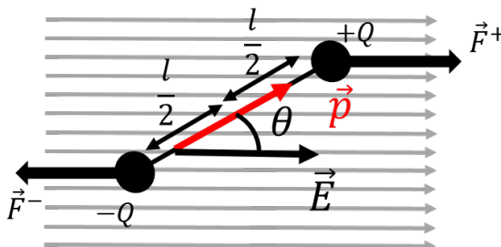
Figure 323: An electric dipole in a uniform electric field.
