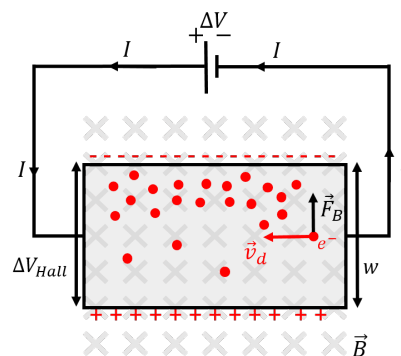
Figure 425: Illustration of the Hall effect, as electrons flow through a slab that is immersed in a magnetic field, the magnetic force pushes them to one side, creating an
