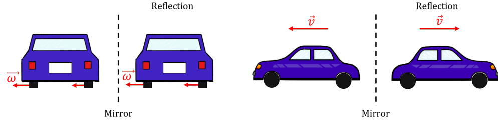
Figure 30: Left: The angular velocity vector for the rotation of the wheels, \vec{\omega} , which points to the left, also points left in the reflection. Right: The velocity vector, pointing to the left, points to the right in the reflection of the car. The angular velocity vector is called an “axial” or “pseudo” vector because it does not change direction under a reflection.
