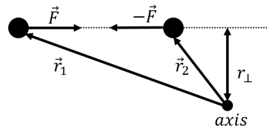
Figure 197: Two particles will exert equal and opposite torques on each other due to Newton's Third Law; the forces exerted by each particle on the other are co-linear and will thus have the same lever arm relative to any point/axis of rotation.
