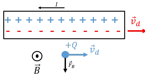
Figure 481: A positive charge, +Q , moving towards the right, near a wire carrying current towards the left, will experience a downwards magnetic force, \vec{F}_B = Q\vec{v}_d \times \vec{B} .
