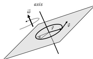
Figure 187: Defining the vector \vec{r} and the angular velocity, \vec{\omega} for a particle with velocity \vec{v} rotating about an axis in a general direction.
