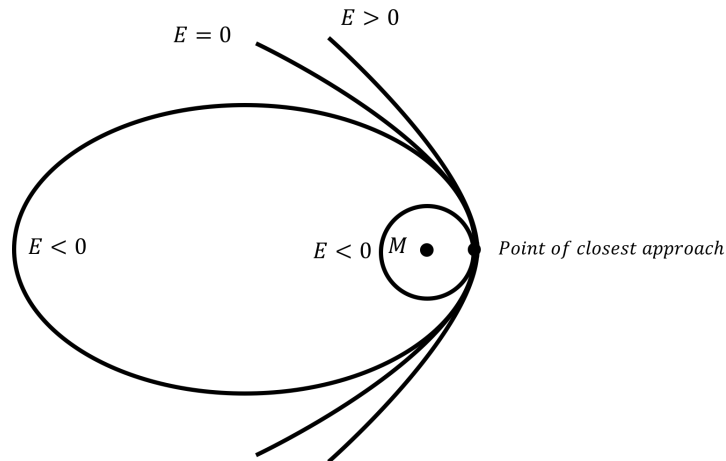
Figure 180: The different possible orbits of m due to the gravitational force of M depend on the mechanical energy, E , of m . The orbits are drawn in a frame of reference where M is at rest.
