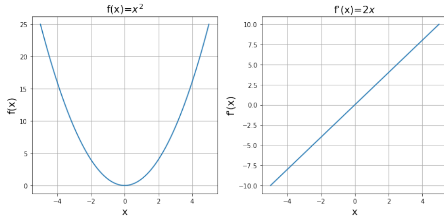
Figure C: f(x) = x^2 and its derivative, f'(x) = 2x plotted for x between -5 and +5 .
