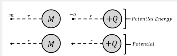
Figure 351: Gravitational potential energy and gravitational potential (left) next to its electrical analogue (right).
