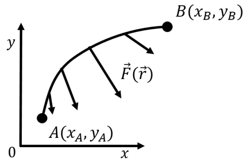
Figure 132: An arbitrary path between two points A and B with a force that depends on position, \vec{F}(\vec{r}) .
