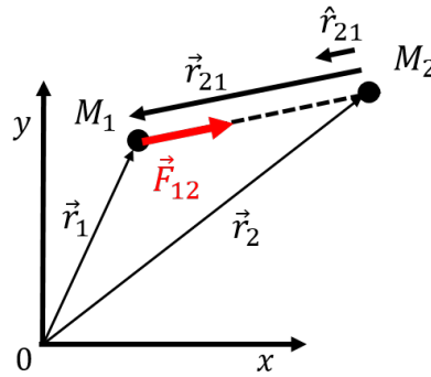
Figure 172: Illustration of the vectors involved in Newton's Universal Theory of Gravity.
