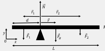
Figure 205: Forces exerted on the plank.
