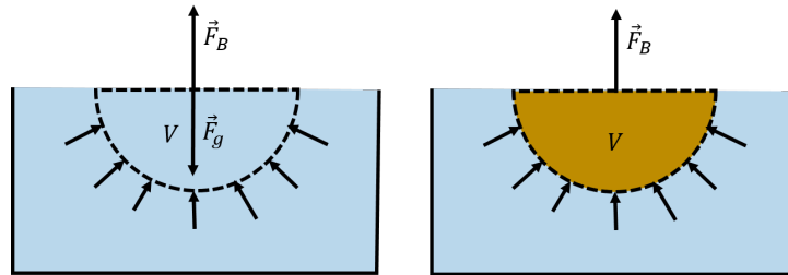
Figure 283: (Left:) The weight of a fluid element, \vec{F}_g , is supported by the net upwards force from the pressure, \vec{F}_B , of the fluid below it. (Right:) If the fluid element is removed and replaced with an object, there will still be the same net upwards force, \vec{F}_B , from the pressure of the fluid, which is now exerted on the object.
