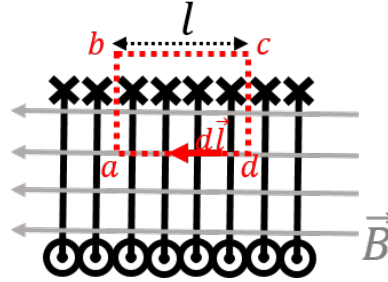
Figure 450: We use Ampère's Law with a rectangular loop to evaluate the strength of the magnetic field inside a solenoid.
