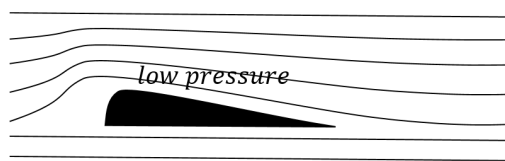
Figure 288: Laminar flow of air around an airfoil. The curvature of the asymmetric airfoil forces the streamlines above the airfoil together, increasing the speed of the air due to the continuity equation, and resulting in a low pressure area.
