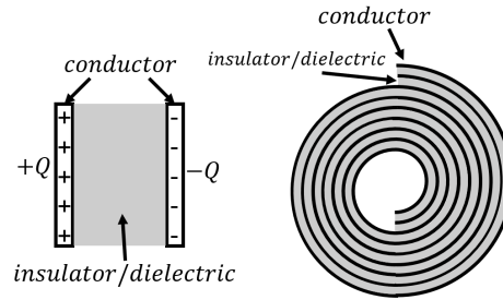
Figure 361: Two examples of capacitors. The left panel shows a “parallel plate” capacitor, and the right panel shows a cylindrically shaped capacitor obtained by “rolling up” a parallel plate capacitor.
