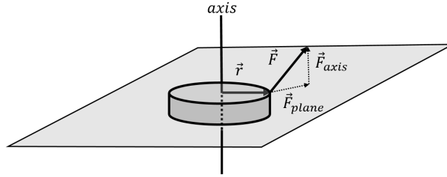
Figure 194: A force exerted on disk that can only rotate about an axis through its centre and perpendicular to its plane. Only the component of \vec{F} that is in the plane perpendicular to the axis of rotation, \vec{F}_{plane} , will contribute to the torque about the axis of rotation.
