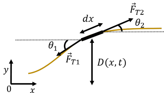
Figure 257: A small section of rope under tension as a wave passes through.
