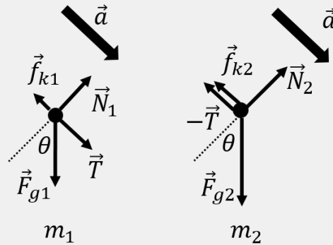
Figure 82: Free-body diagram for the blocks m_1 and m_2 from Figure 15
