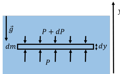
Figure 275: Pressure gradient from gravity on an infinitesimal fluid element.
