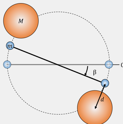
Figure 238: Two very large spheres are placed near each of the small masses on the torsional pendulum (top view). At the new equilibrium, each small mass is a distance d from the nearest large mass.
