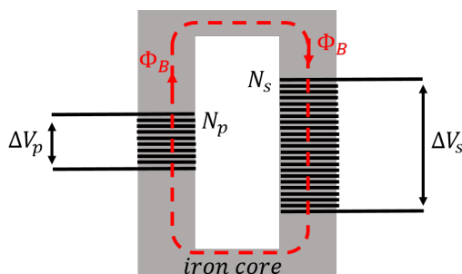
Figure 466: A transformer converts a primary alternating voltage, \Delta V_p , to a secondary alternating voltage, \Delta V_s . The magnetic flux produced in one coil is transmitted by an iron core to the secondary coil, where a different voltage is induced, depending on the ratio of the number of windings in each coil.
