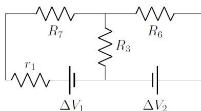
Figure 394: The resistors R_4 and R_5 in parallel from the circuit in Figure 17 have been combined into the effective resistor, R_7 , to simplify the circuit.
