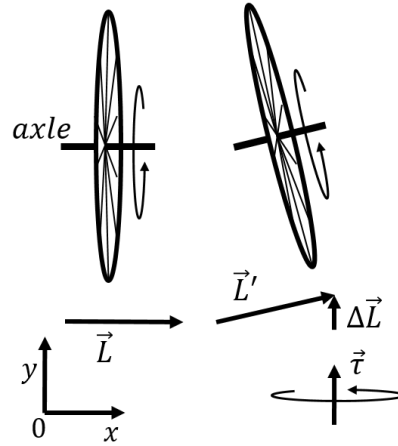
Figure 222: A wheel rotating on an axle, with a horizontal angular velocity (left). If you try to tilt the axle as shown in the right panel, changing the angular momentum of the wheel, you will also need to exert a torque in the vertical direction (shown at the bottom right).
