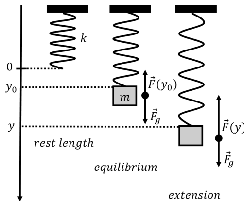
Figure 232: A vertical spring-mass system.
