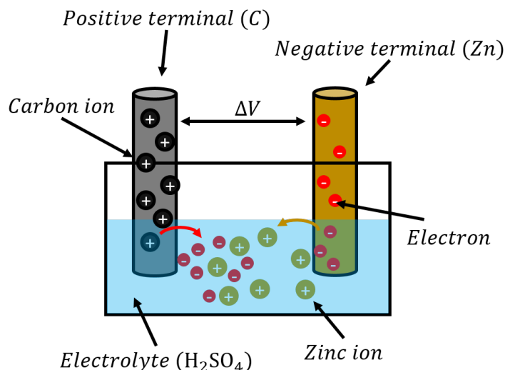
Figure 377: A simple electric cell, where zinc ions dissolve in sulfuric acid leaving electrons on the metal.
