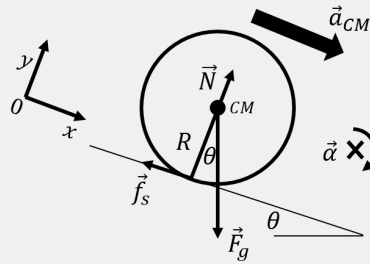
Figure 219: The forces on the disk rolling without slipping down an incline.
