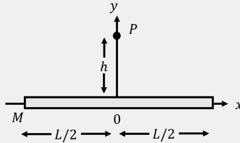
Figure 183: A thin rod of mass M and length L produces a gravitational field at a point P located above the midsection of the rod.
