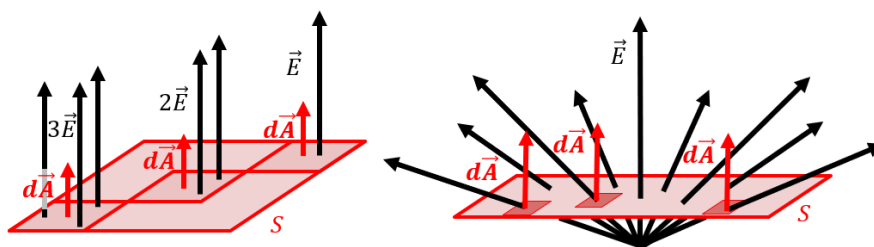
Figure 327: Examples of surfaces that need to be sub-divided in order to determine the net flux through them. The surface on the left must be subdivided because the electric field changes magnitude over the surface, whereas the one on the right needs to be subdivided because the angle between \vec{E} and d\vec{A} is not constant (and the magnitude of \vec{E} also changes along the surface).
