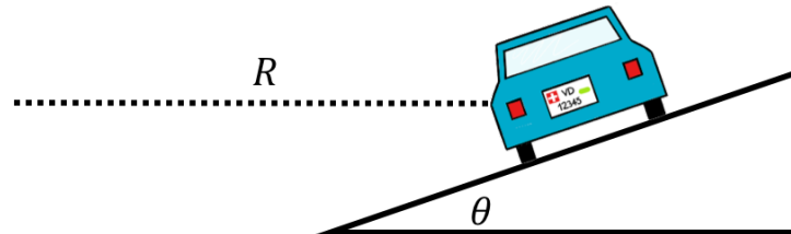
Figure 114: A car moving into the page and going around a banked curved so that it is turning towards the left (the centre of the circle is to the left).
