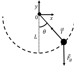
Figure 234: A simple pendulum which oscillates in a vertical plane.
