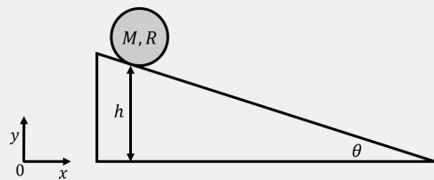
Figure 216: A disk rolling without slipping down an incline.
