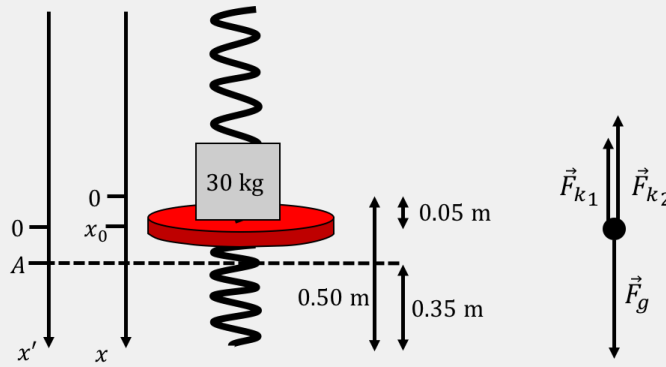
Figure 240: The forces acting on the platform and our new coordinate system.
