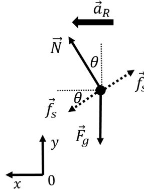
Figure 115: Free-body diagram for the forces on the car. The direction of the force of static friction cannot be determined, as it depends on the acceleration of the car, so it is shown twice (with dotted lines).
