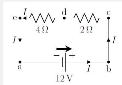
Figure 383: Two resistors connected in series with a battery.
