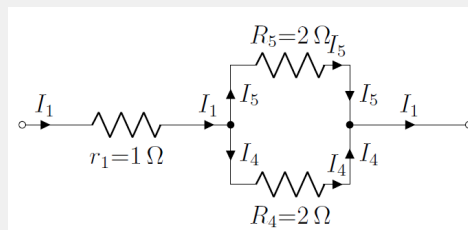
Figure 399: The components of the effective R_8 resistor from Figure 22 . The current, I_1 , coming from the battery goes through r_1 and then splits up.
