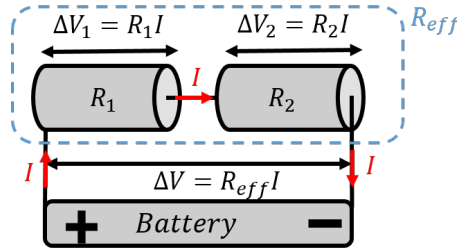
Figure 371: When two resistors are connected in series, the same current flows through each resistor.
