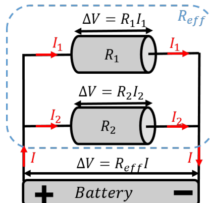
Figure 373: When two resistors are connected in parallel, the same voltage is applied across each resistor.
