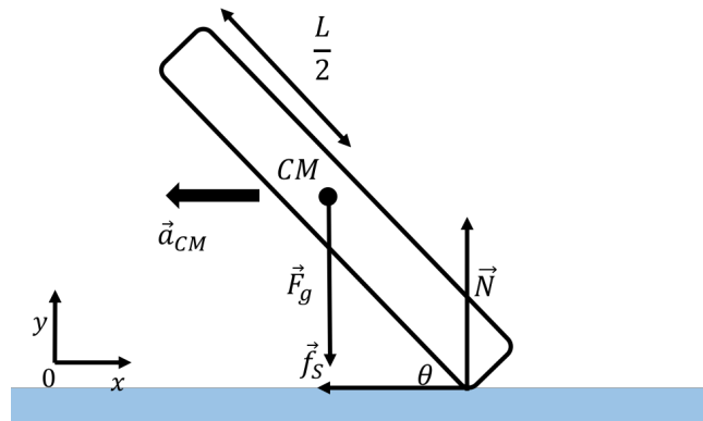
Figure 207: Forces on the speed skater from Figure 22.
