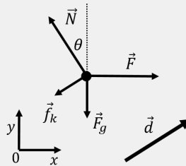
Figure 137: Free-body diagram for the crate on the incline.
