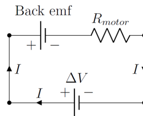
Figure 462: A simple circuit illustrating how a motor, with resistance, R_{motor} , will generate a “back emf”, equivalent to a battery that produces a voltage in the direction to oppose the current from the actual battery that is powering the motor, \Delta V .
