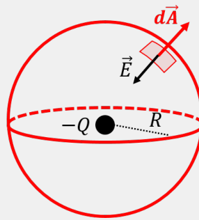
Figure 330: Calculating the flux through a spherical surface.
