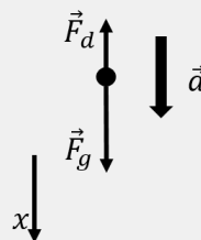
Figure 105: Free-body diagram for a block free-falling with drag.
