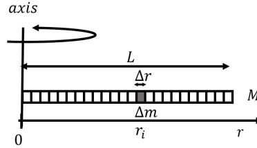
Figure 201: A rod of length L and mass M being rotated about an axis perpendicular to the rod that goes through one of its ends.
