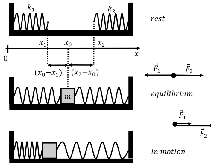
Figure 233: A mass attached to two different springs.
