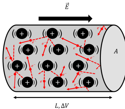
Figure 367: Electrons moving inside a conductor only “drift” on average in the direction anti-parallel to the electric field. In reality, they constantly collide with atoms in the material, transferring their kinetic energy into thermal energy of the conductor.
