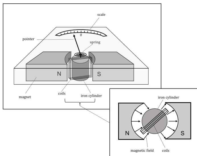
Figure 428: Illustration of a galvanometer. Current passes through the coil, and the coil rotates due to the torque from a magnetic field created by a permanent magnet. The torque from the magnetic force is balanced by a torsional spring.
