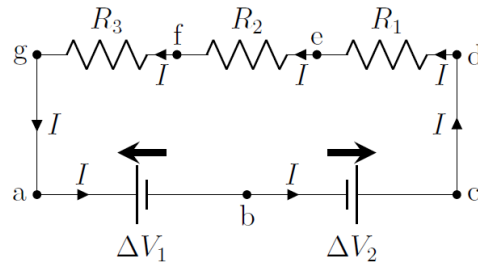
Figure 390: A loop with 2 batteries and 3 resistors.
