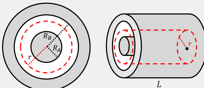
Figure 364: Solving for E between two cylinders using Gauss' law.
