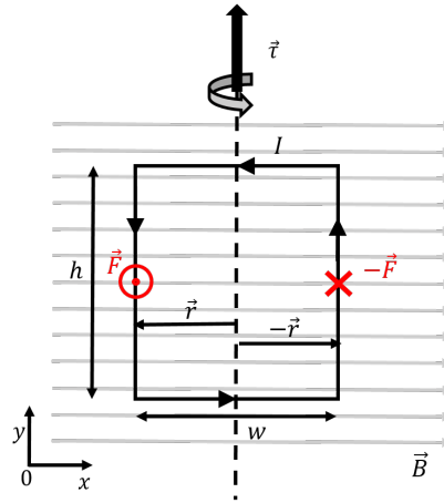
Figure 422: A rectangular loop carrying counter-clockwise current in a uniform magnetic field.
