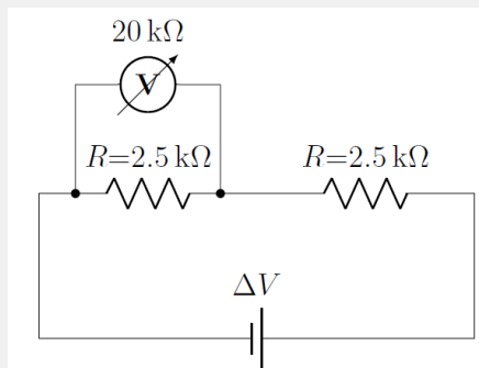
Figure 410: A circuit with a battery of unknown voltage.
