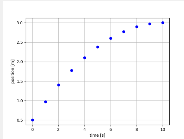
Figure 43: Position vs. time for a rock sliding with friction decelerating the rock.
