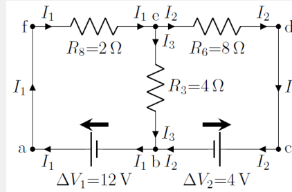
Figure 398: Simplified version of the circuit in Figure 21.
